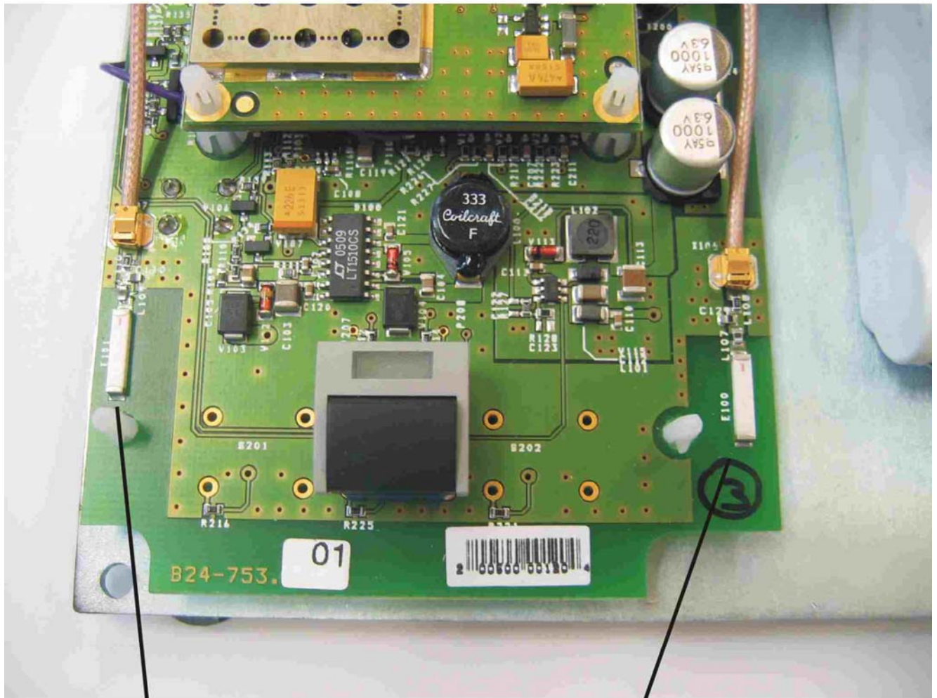
Duplex-Antenna TX / RX
