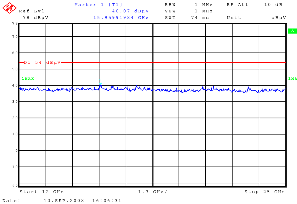
Plot 4: 12- 25 GHz (receiver)
