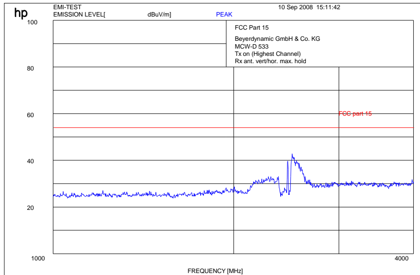
Carrier notched with 2.4 GHz rejection filter
