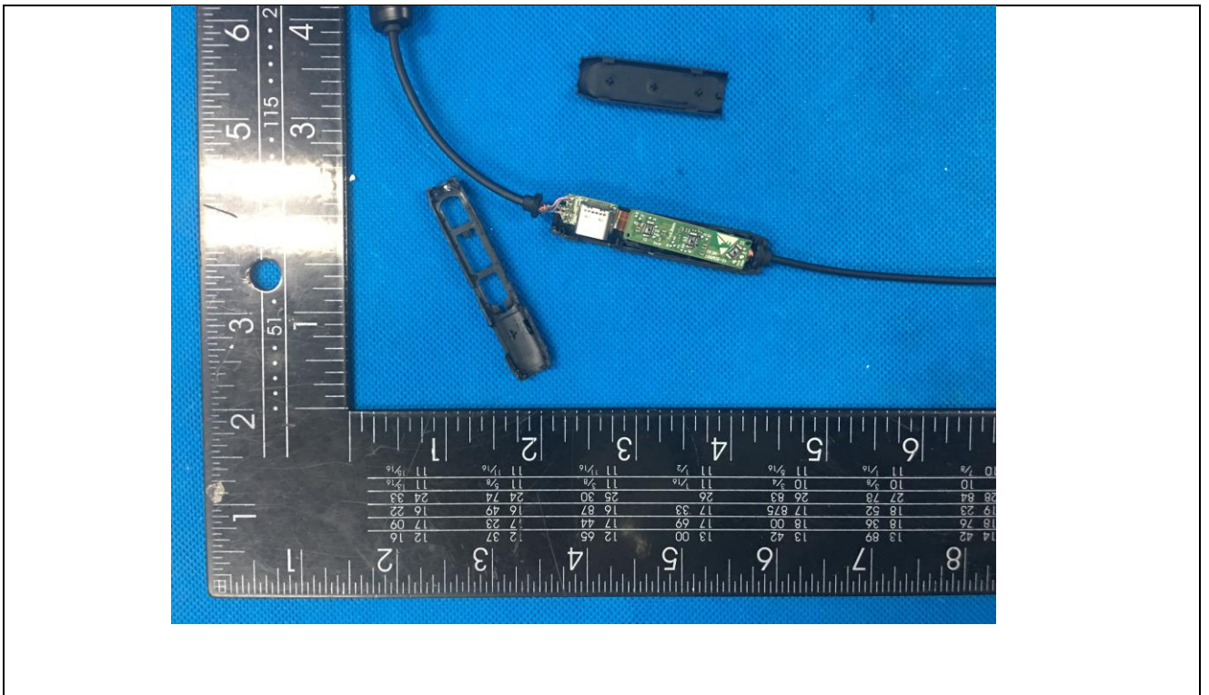
Details of: Internal view of volume setting enclosure
