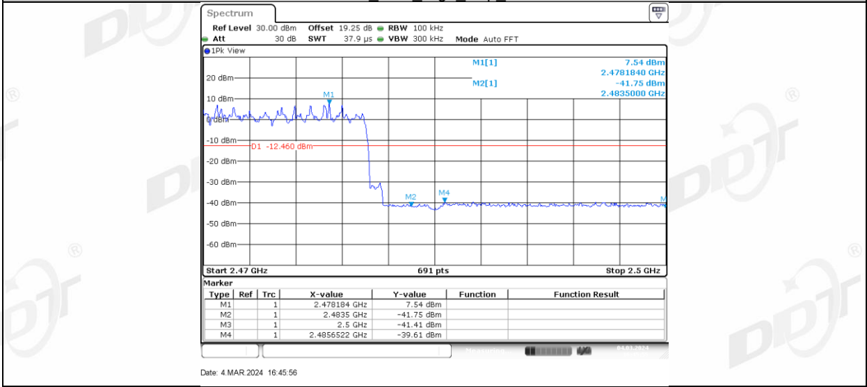
3DH5_Ant1_High_Hop_2480
