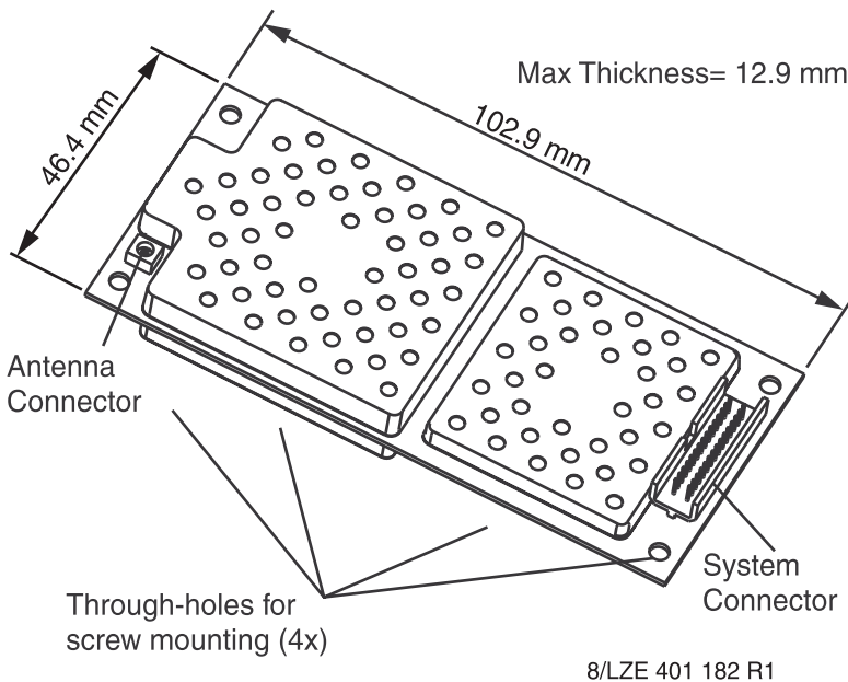
Figure 7 Main dimensions for the M3090 radio modem.
