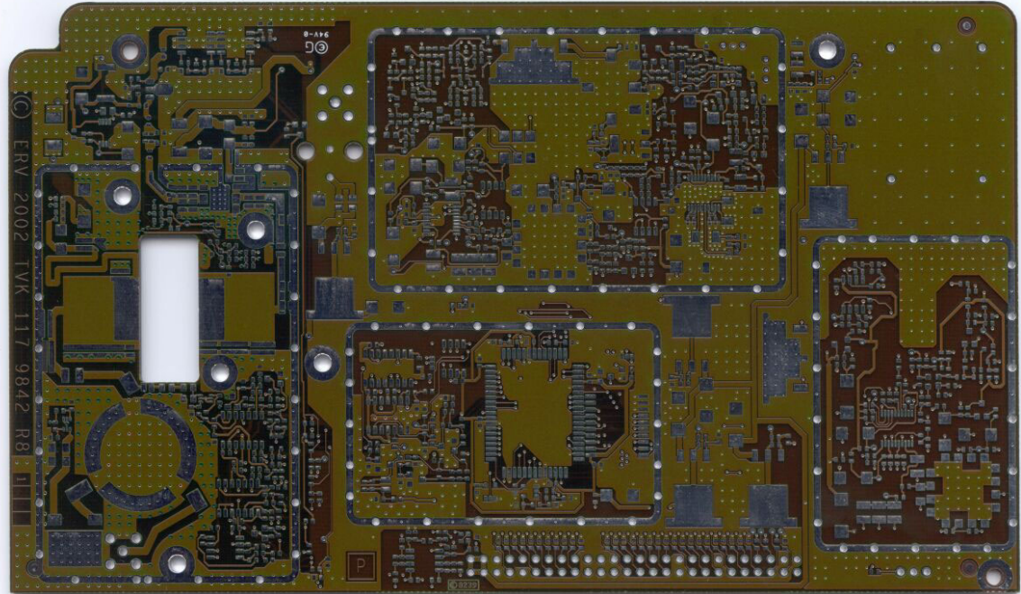
BRU19 FRB (radio board) blank PCB, top side
