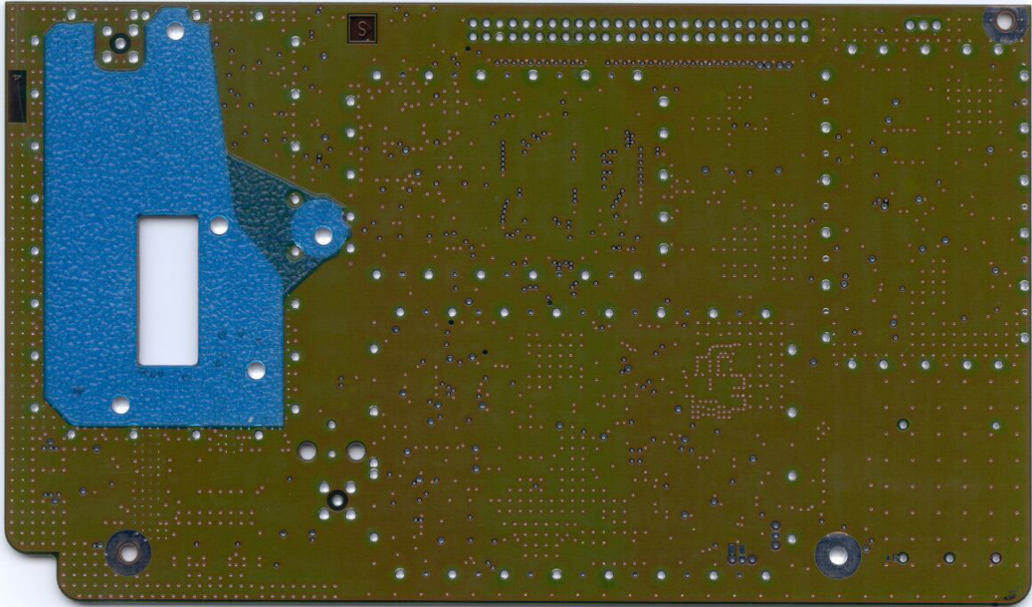
BRU19 FRB (radio board) blank PCB, bottom side
