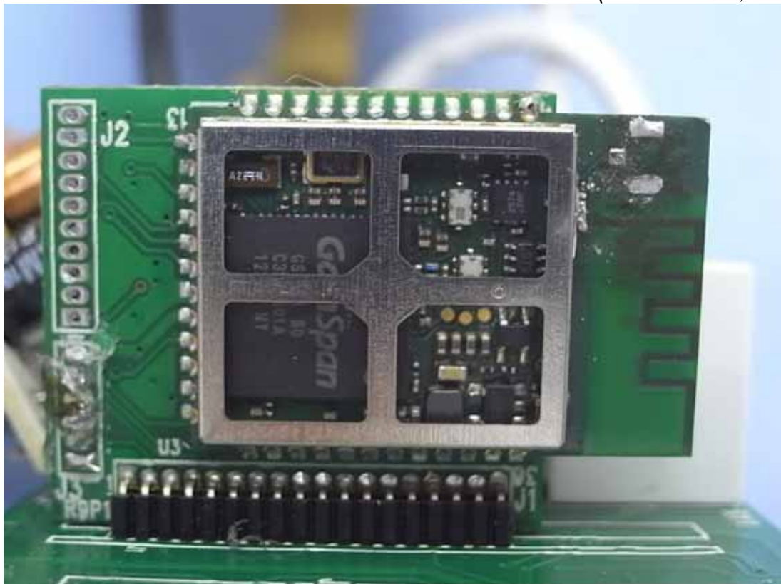
Photo 10 Internal View (Wi-Fi Module, Front View)
