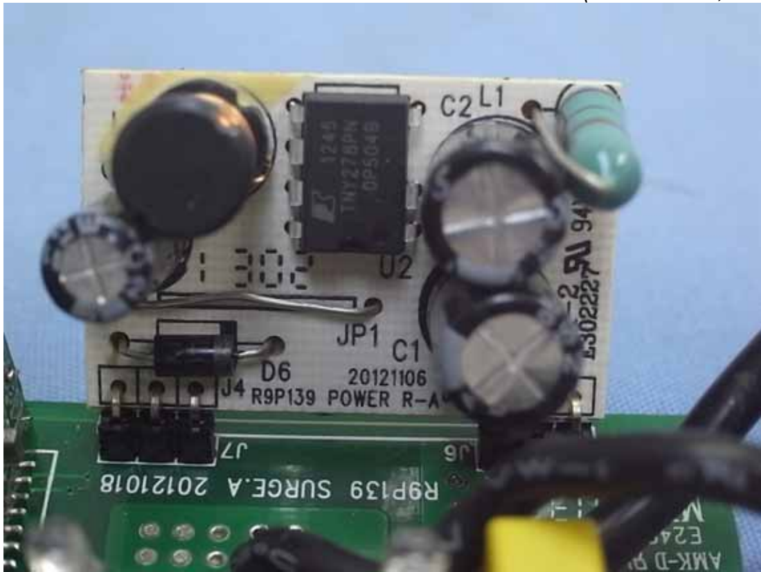
Photo 8 Internal View (Power Board, Back View)
