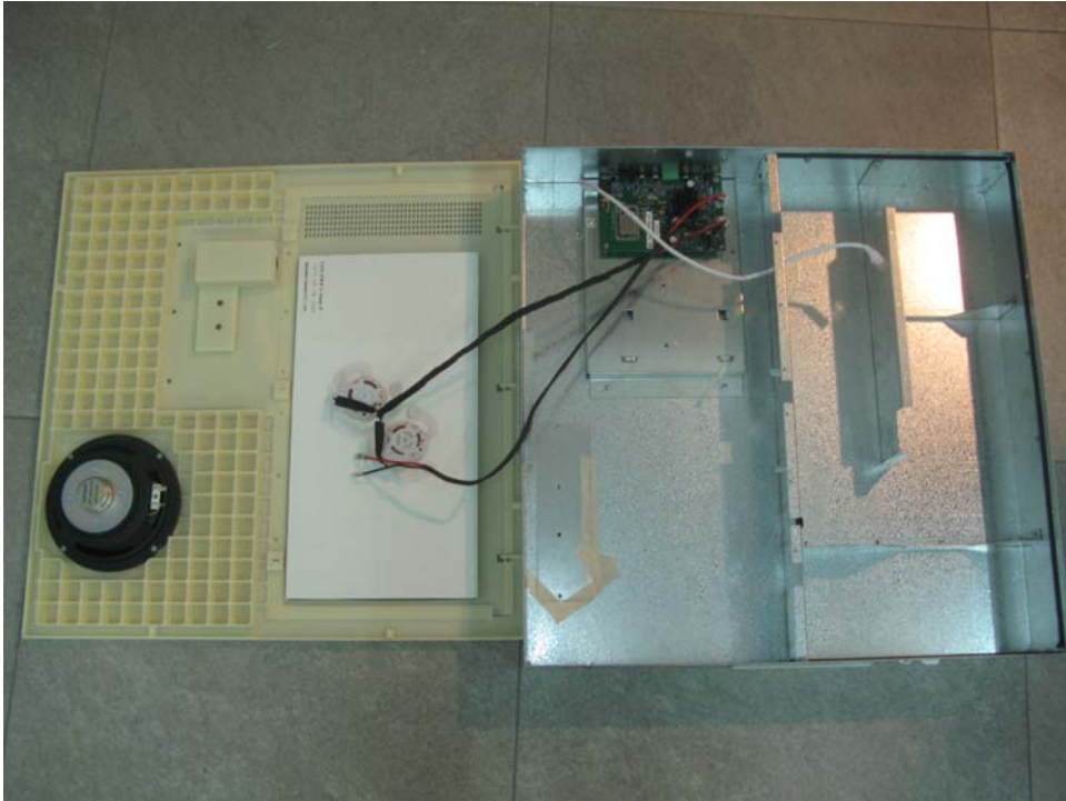
Classroom Audio System assembly
