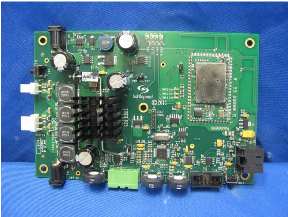
Classroom Audio System Main PCB comp side (View 1)
