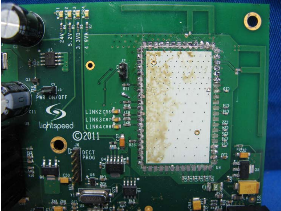
Classroom Audio System Main PCB comp side (View 2)
