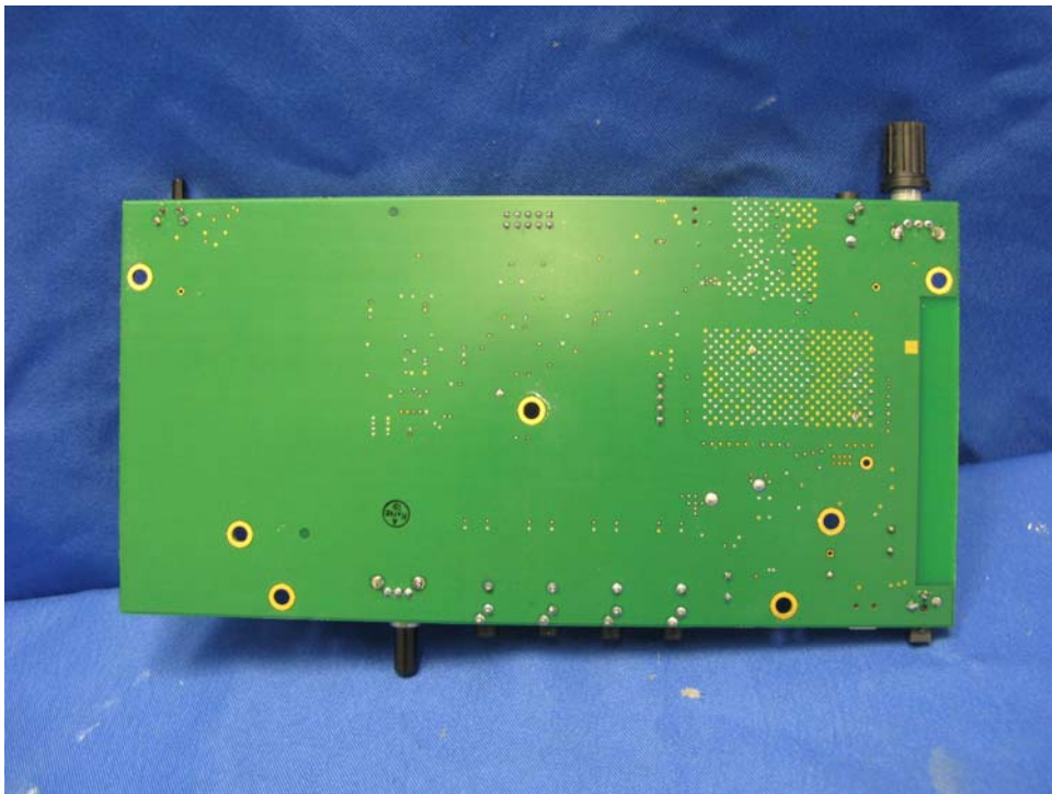
Media Connector Main PCB solder side
