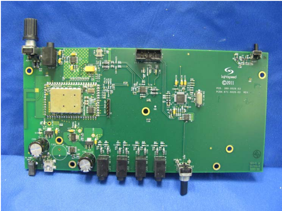
Media Connector Main PCB comp side (view 1)
