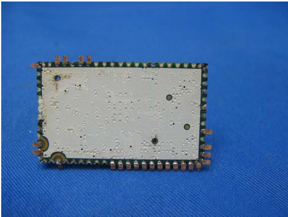
Media Connector Oscillator PCB comp side (view 2)
