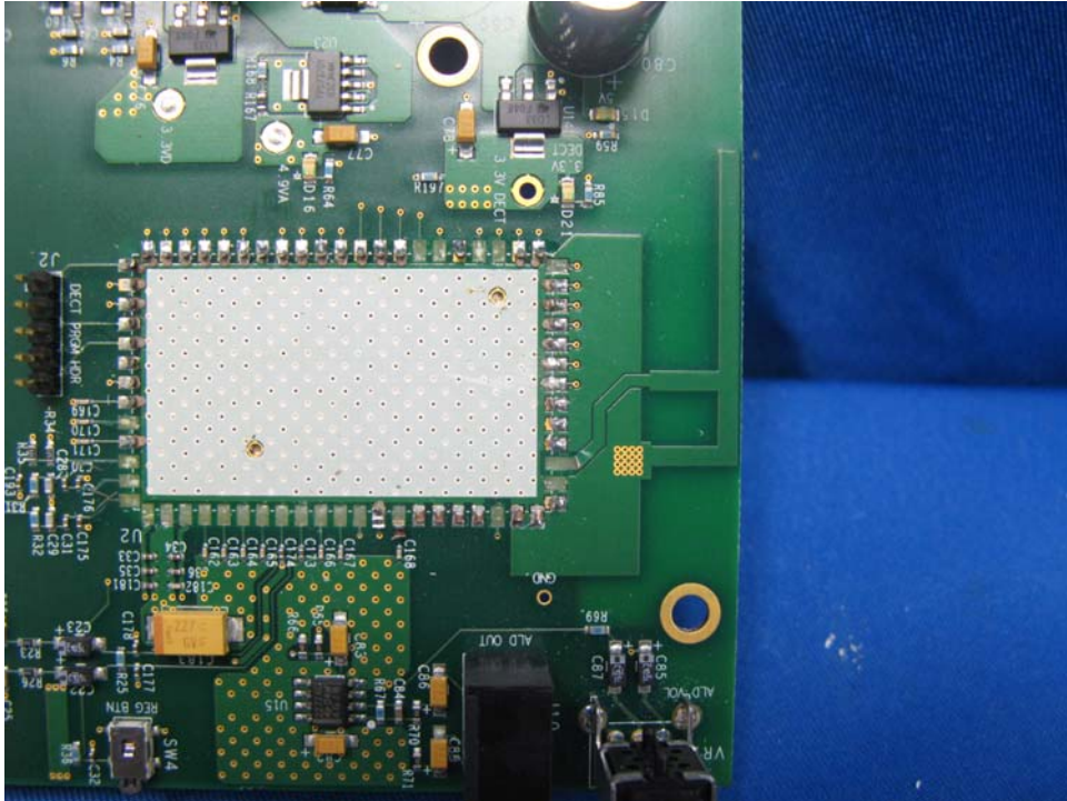
Media Connector Main PCB comp side (view 2)
