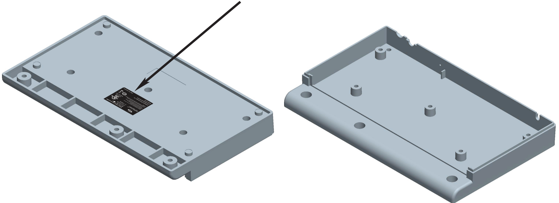
Bottom side of 395-0019-01 Media Connector(MC)
