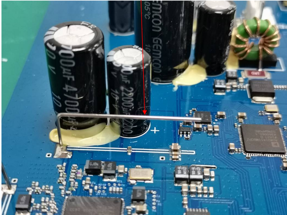
Antenna 0
