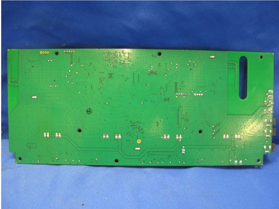
Base Station Main PCB solder side
