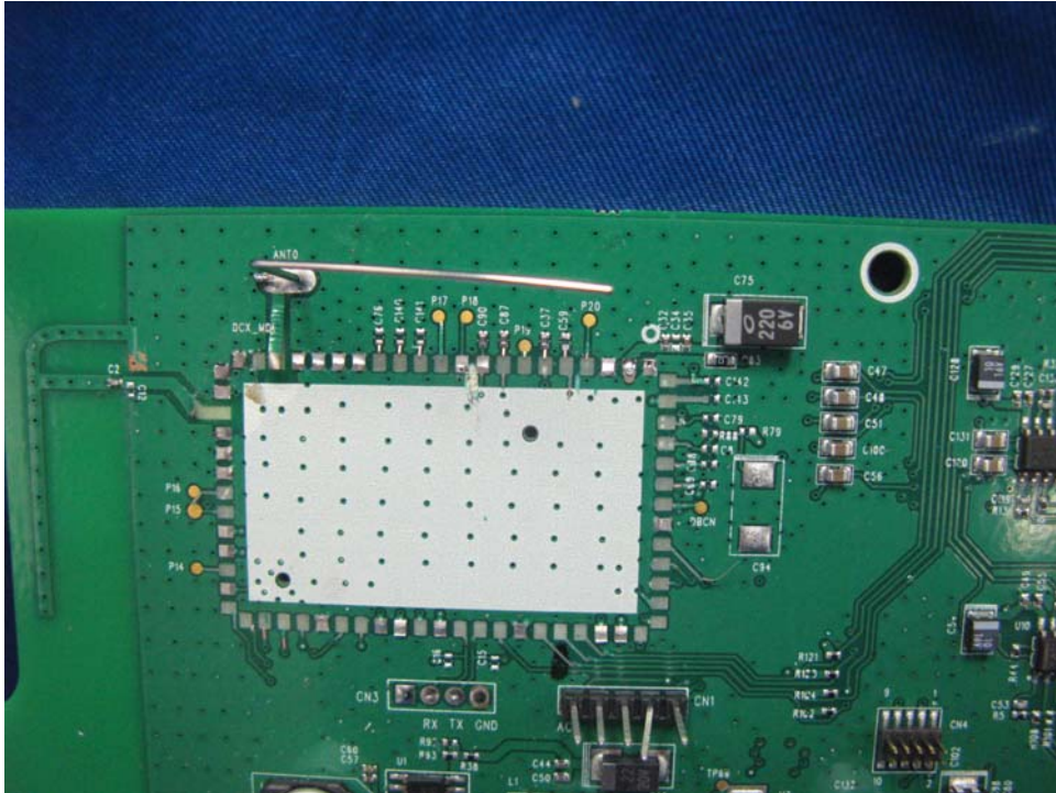
Base Station Oscillator PCB comp side (View 3)
