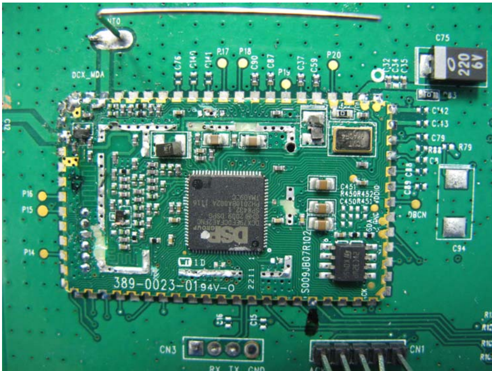
Base Station Oscillator PCB comp side (View 1)
