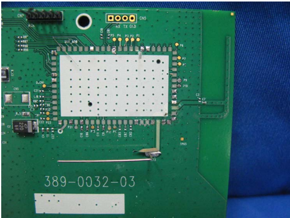
Base Station another Oscillator PCB comp side (View 2)
