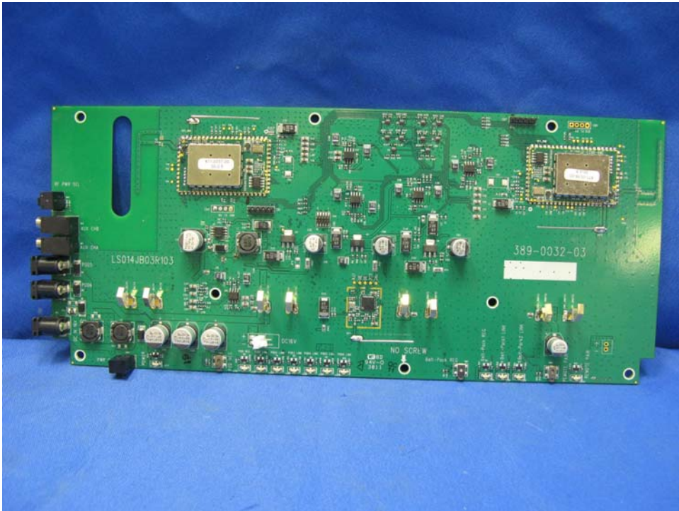
Base Station Main PCB comp side
