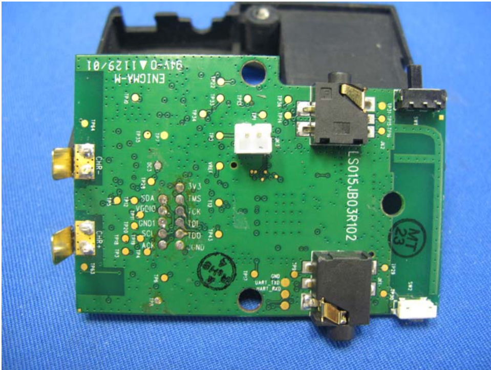
Belt-Pack Main PCB solder side
