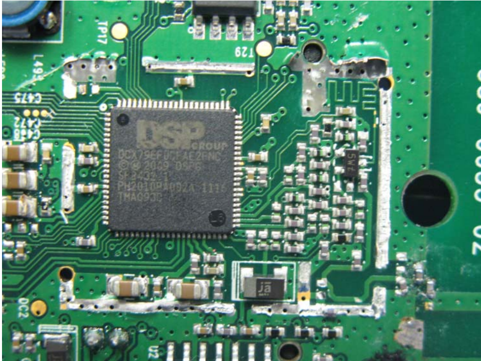
Belt-Pack Oscillator PCB comp side
