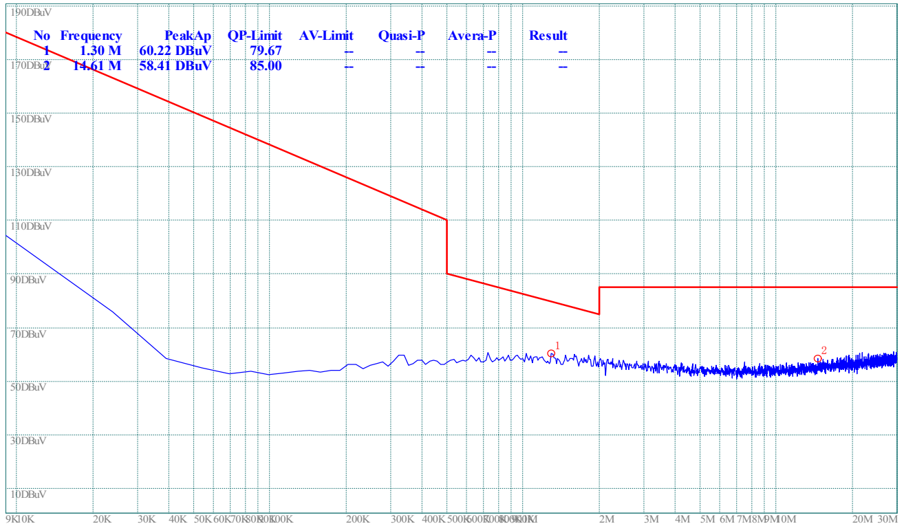
(Plot B.0: 9kHz to 30MHz @ GFSK, channel 39)
