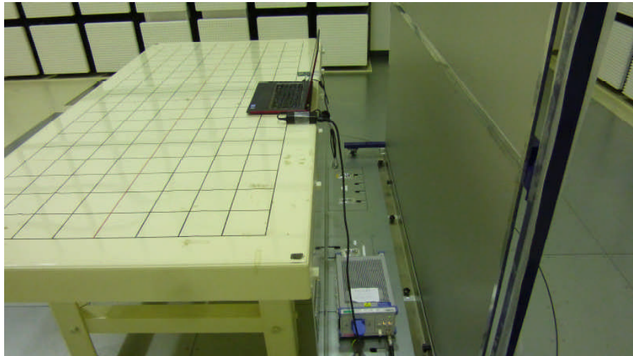
Photo4 Test Setup for Conducted Test_2 (Back)
