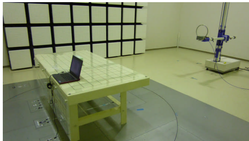
Photo2 Test setup for below 30 MHz ( Back )
