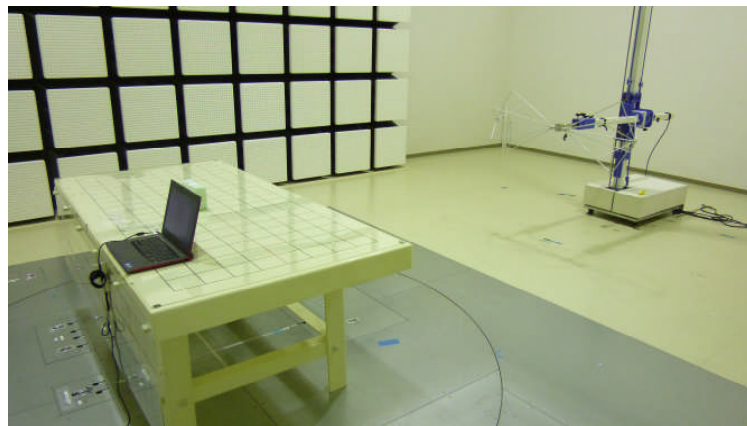
Photo4 Test setup for above 30 MHz ( Back )
