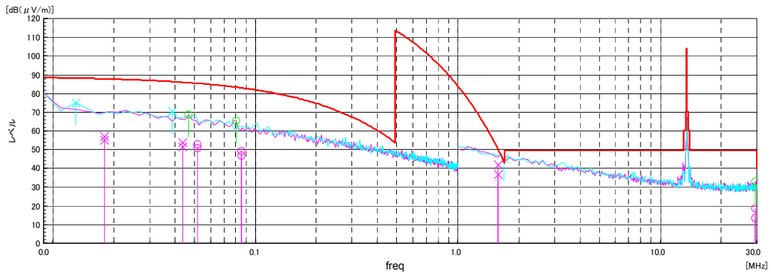
Figure 5 Below 30MHz Radiated Spurious Emission, Out-of-Band Plot
