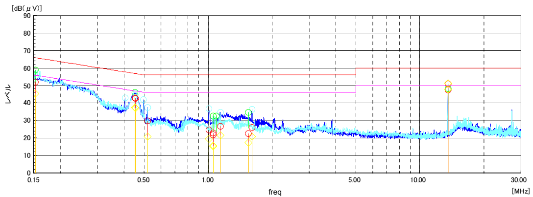
Figure 7 Line-Conducted Test Plot
