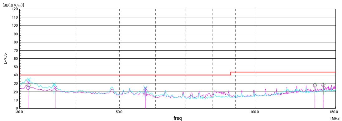
Figure 6 Above 30MHz Radiated Spurious Emission, Out-of-Band Plot
