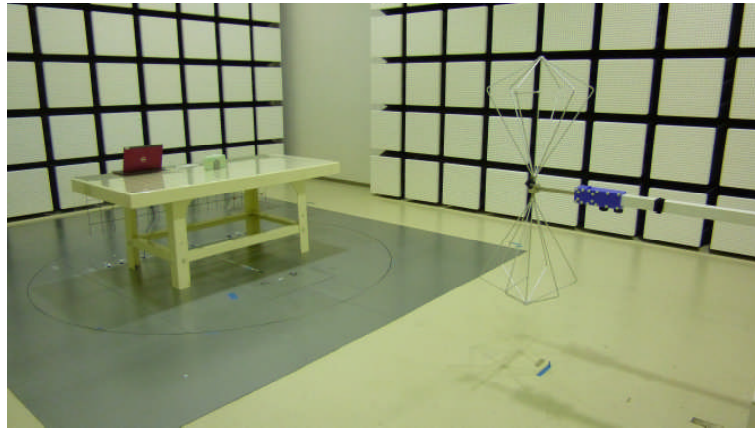
Photo3 Test setup for above 30 MHz ( Front )
