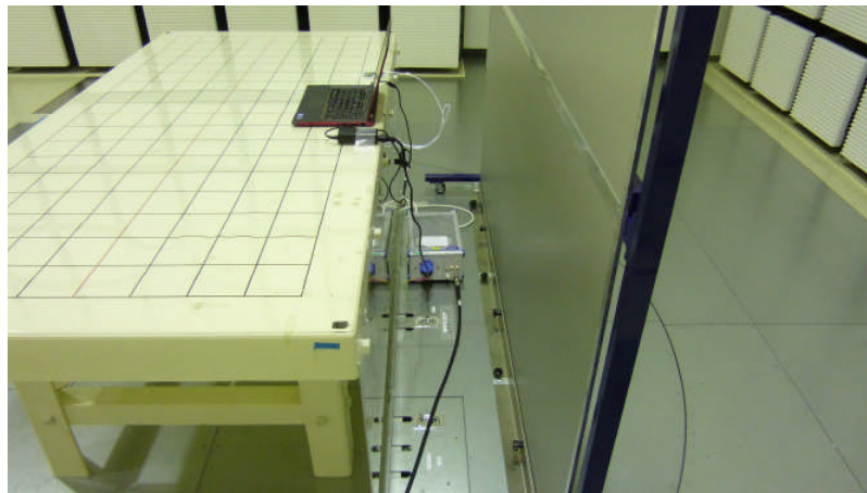
Photo6 Test Setup for Conducted Test_2 (Back)
