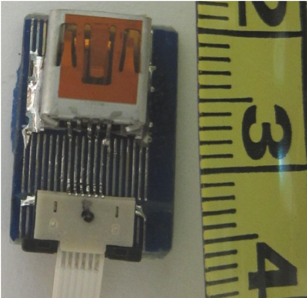
Sub-Board PCB Component Side
