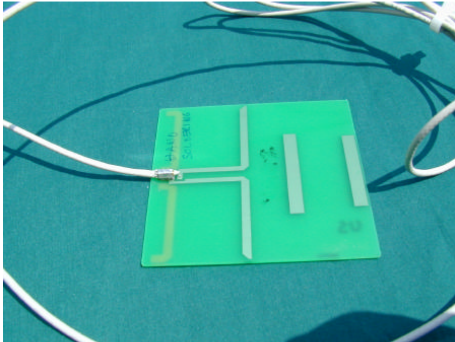
Dipole Antenna
