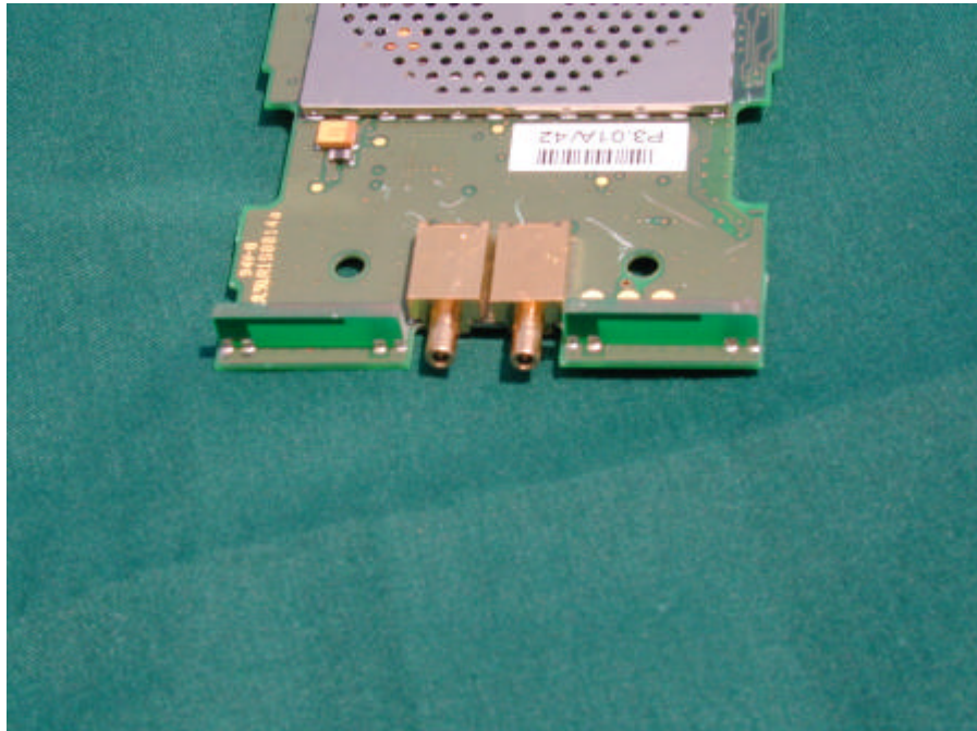
PCB with internal antenna & External Antenna Connection
