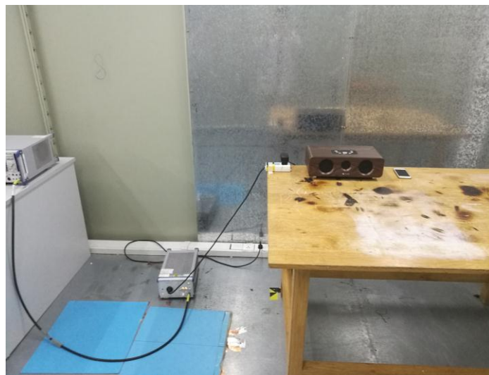
Conducted Emission
