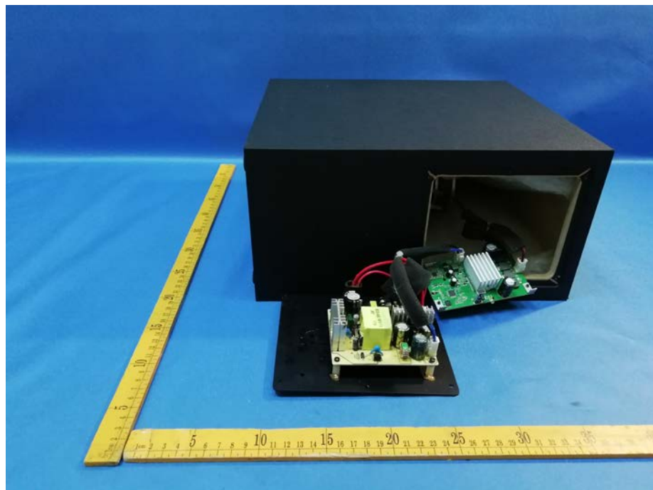
Power board 2:
