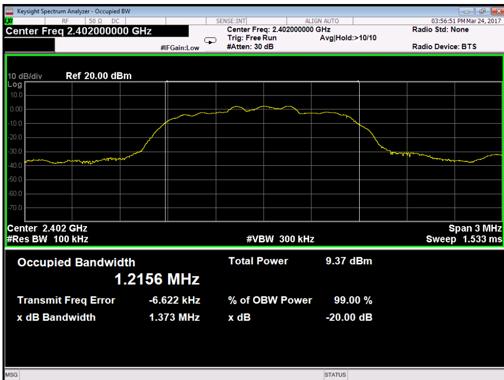
0 Channel @ 8-DPSK
