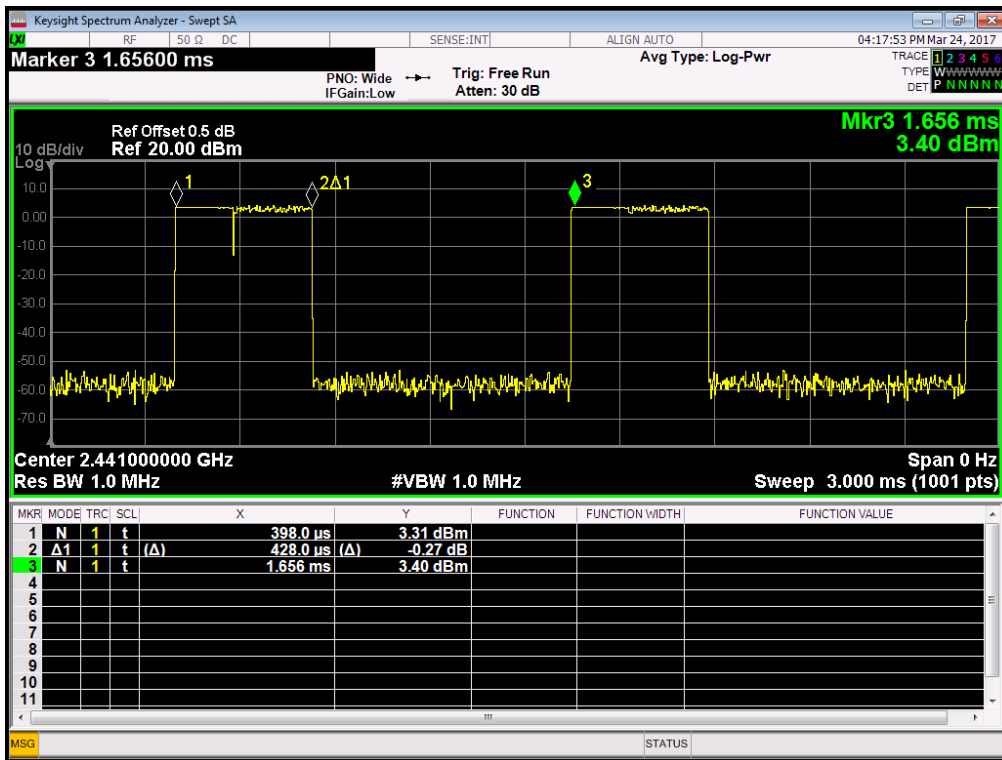
39 Channel @ 3DH1
