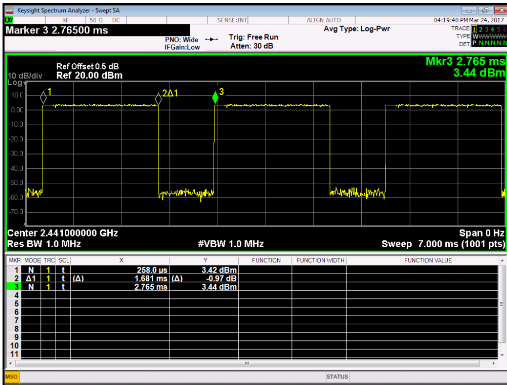
39 Channel @ 2DH3
