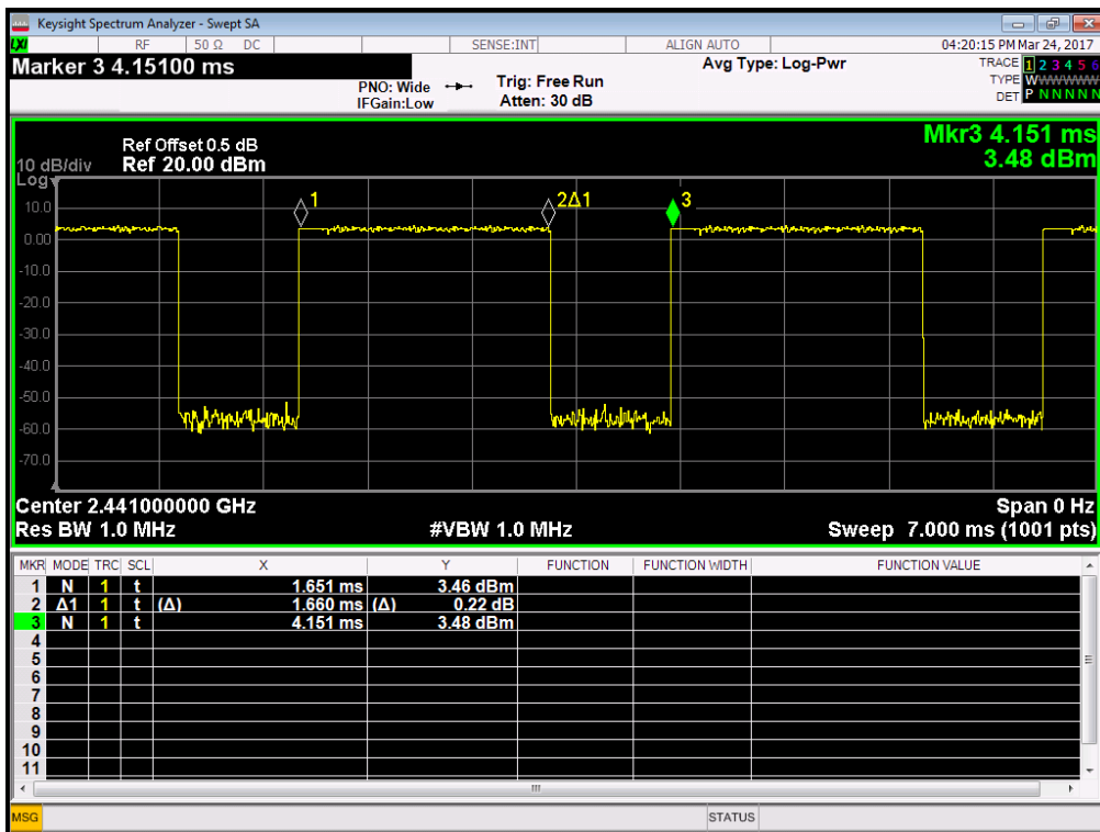
39 Channel @ 3DH3
