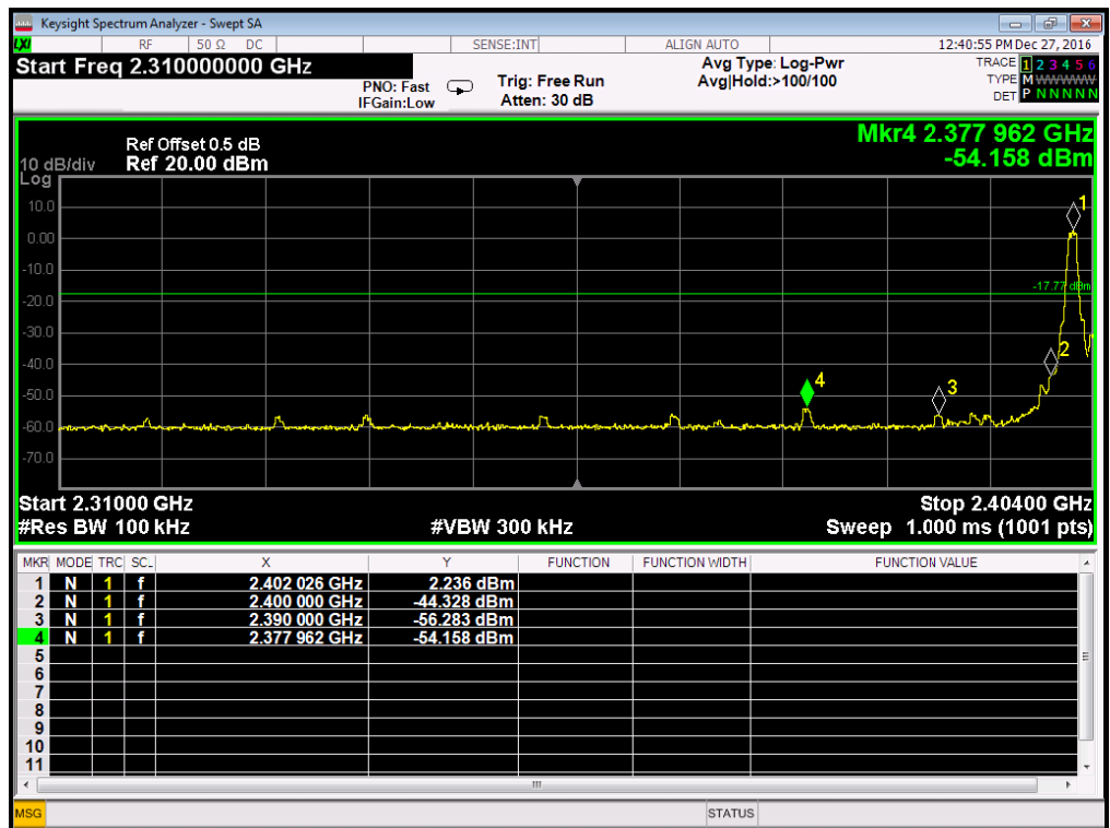
Low Band Edge Plot on Channel 0
