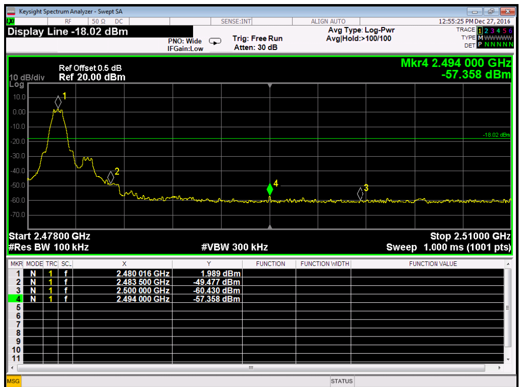
High Band Edge Plot on Channel 39
