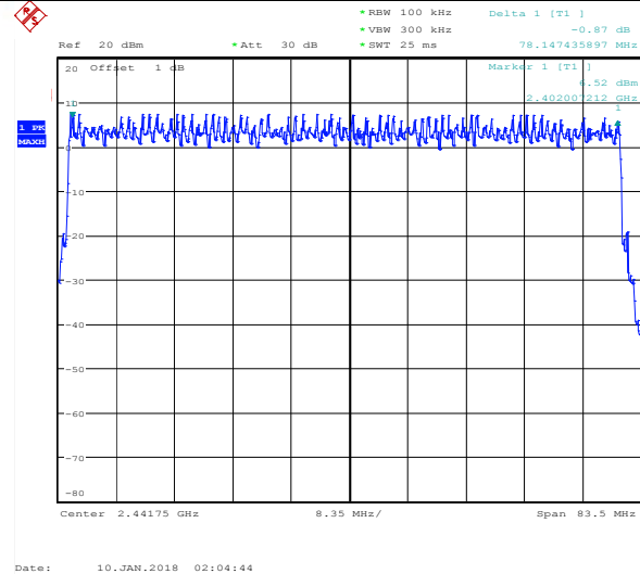
8DPSK Modulation
