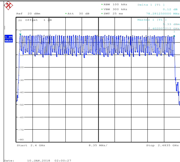
GFSK Modulation
