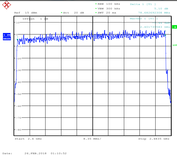
8DPSK Modulation
