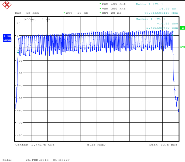
GFSK Modulation
