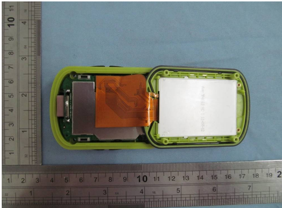
OPEN VIEW OF EUT-1
