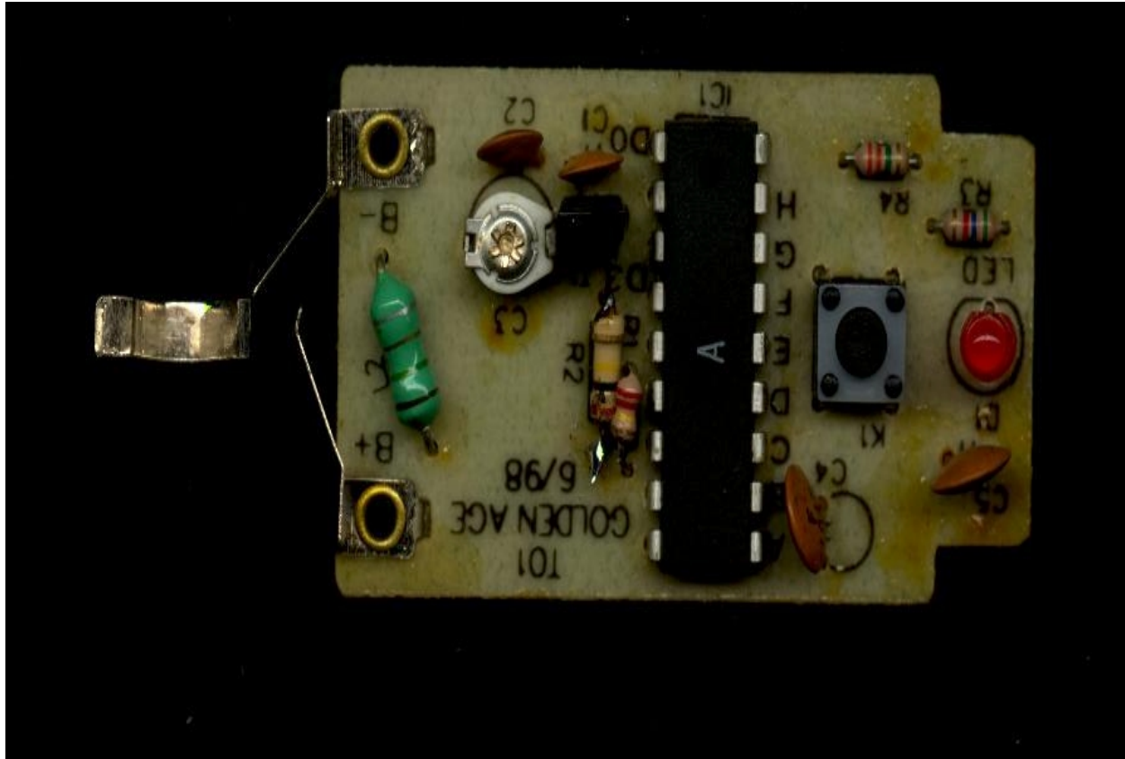
C. Main board component side (Remote control)
