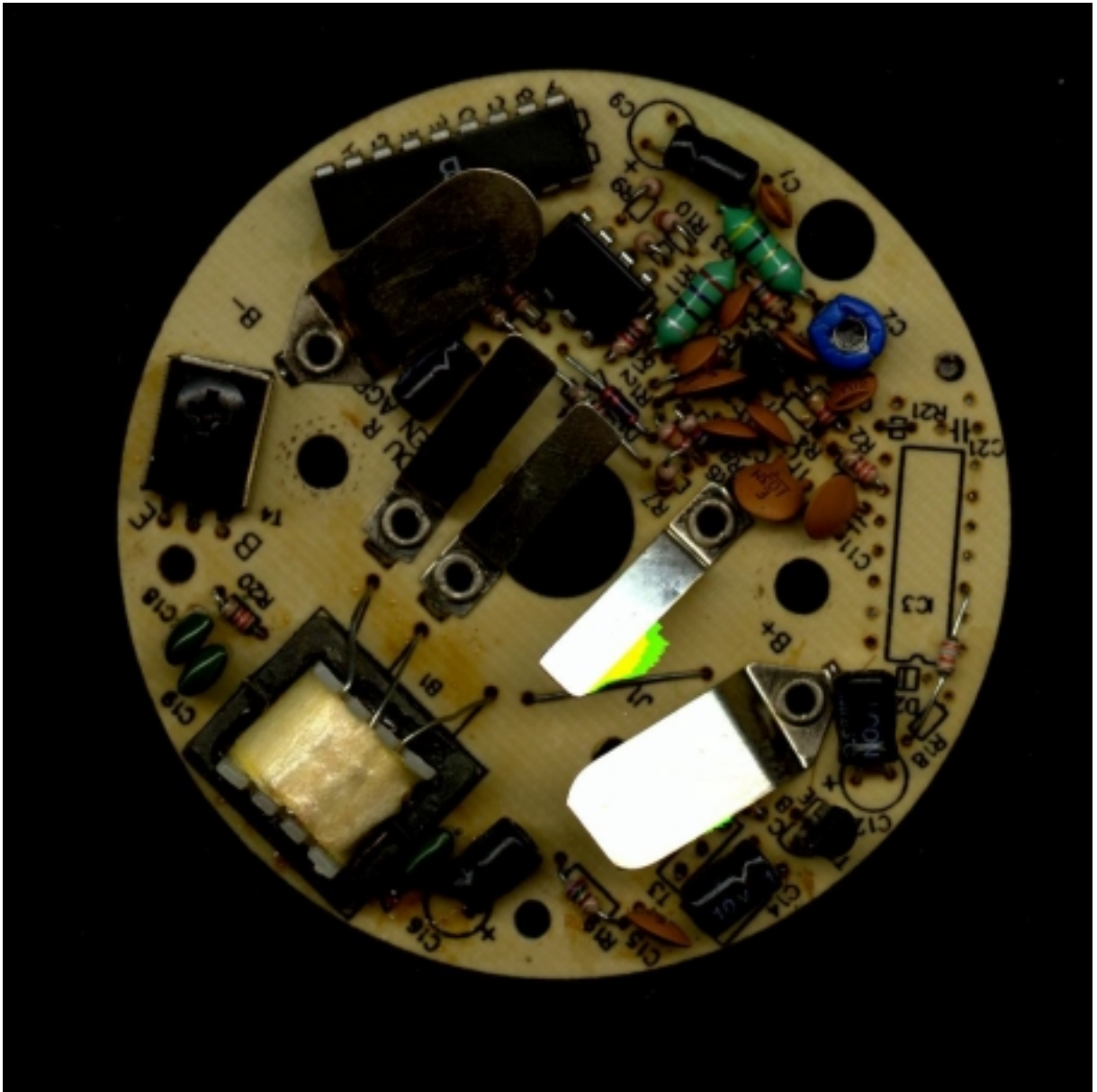
A. Main board component side (Lampstand)
