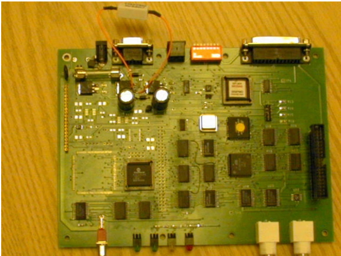
RP-301 Top Side
