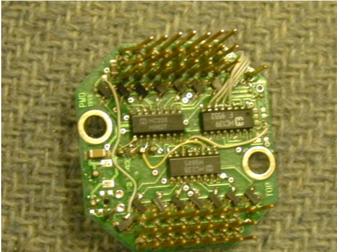
MX-301 PCB – Top View
