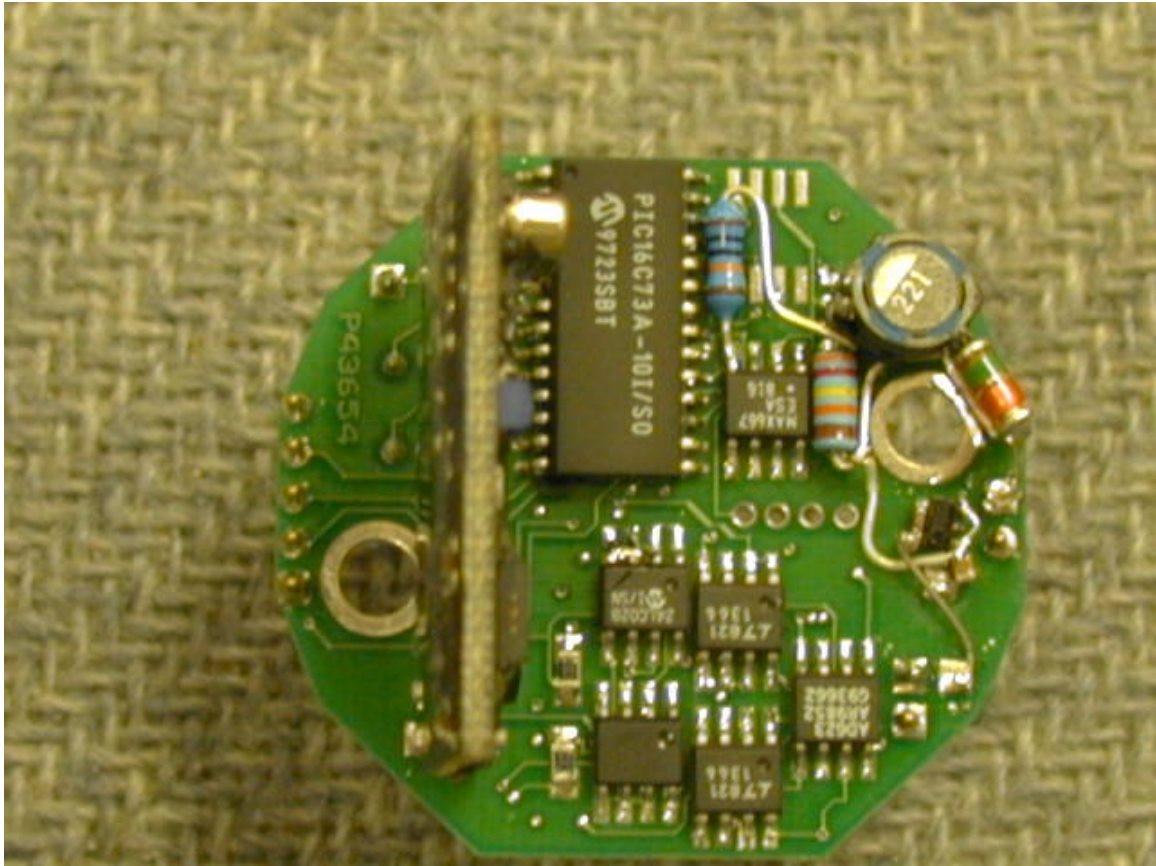
TP-301 PCB – Bottom View
