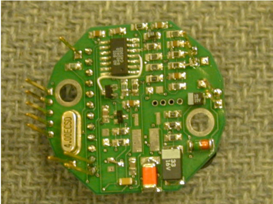
TP-301 PCB – Top View
