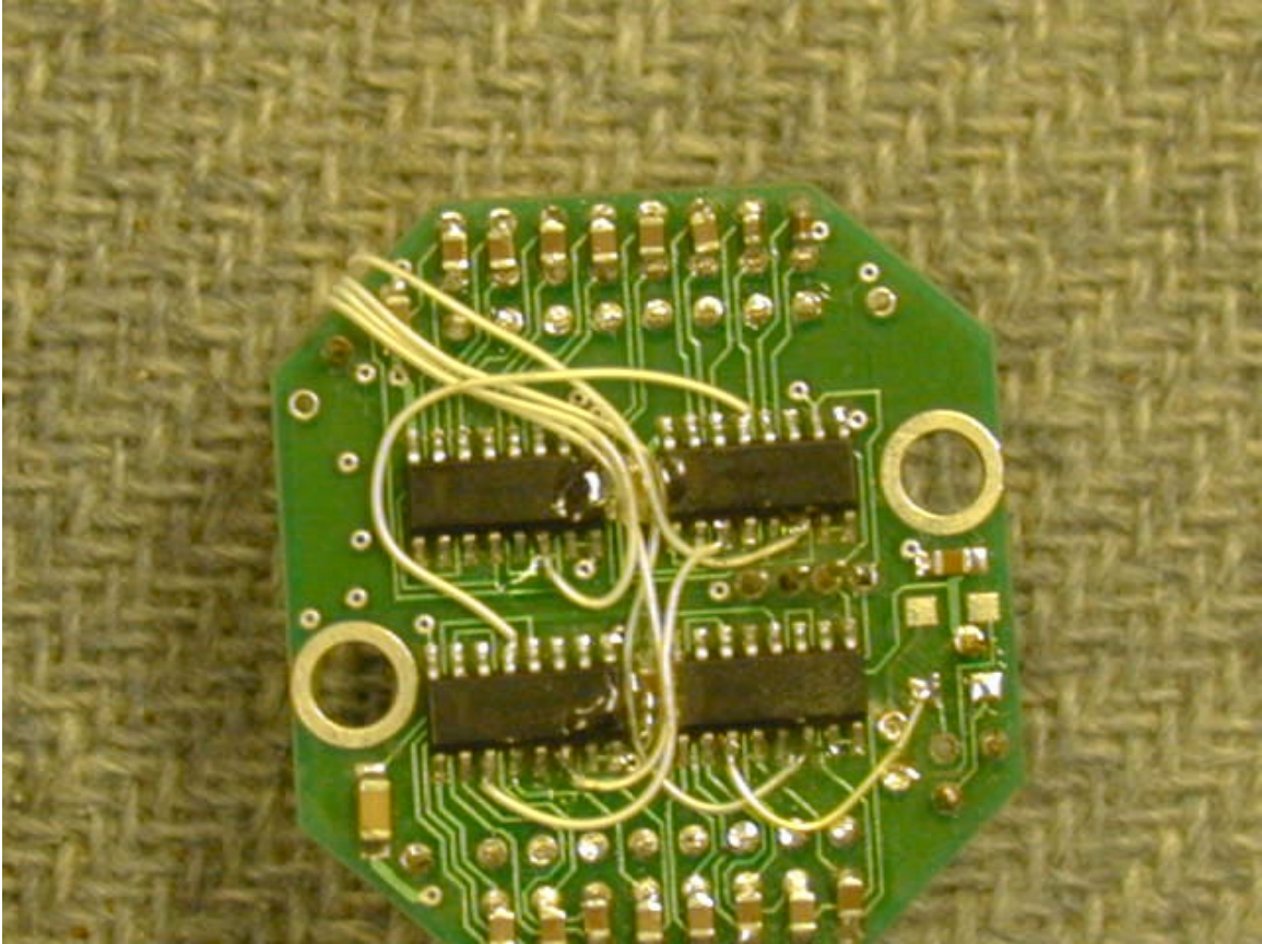
MX-301 PCB – Bottom View
