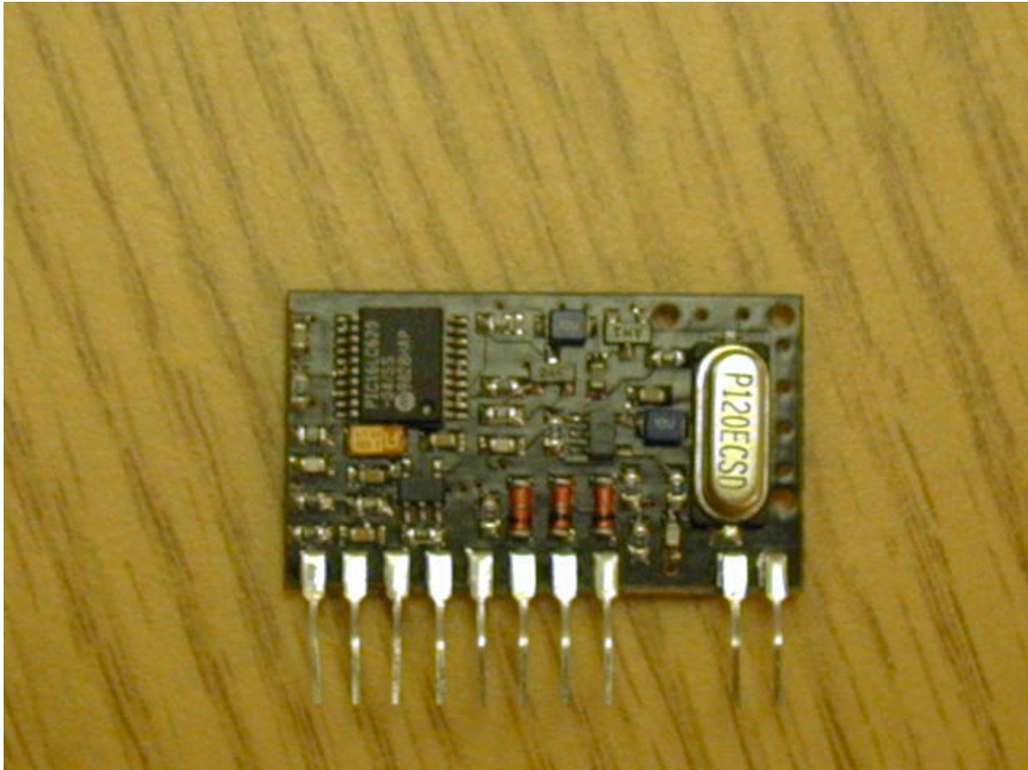
Linx HP-TXM PCB Top View
