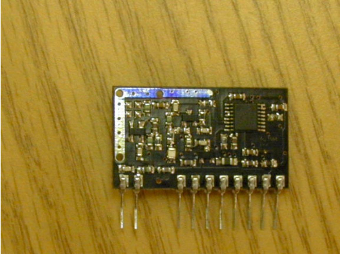
Linx HP-TXM PCB Bottom View
