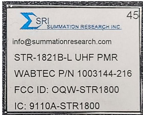
Figure 1 STR-1821B-L Label
