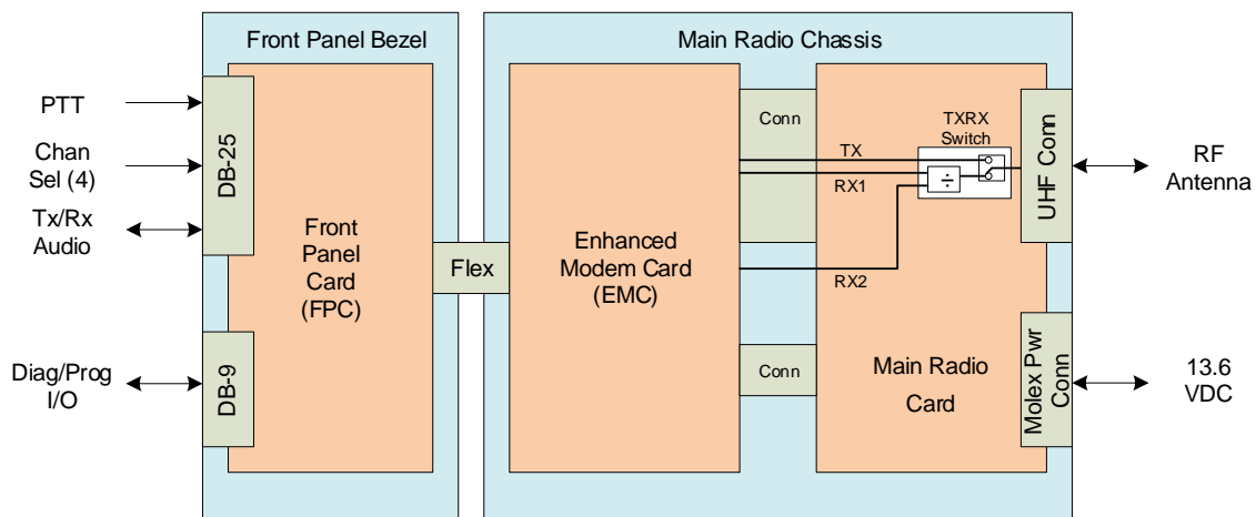
System Overview, Dual Receive Channel Model STR-1821A
