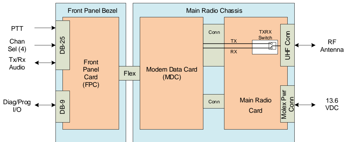
System Overview, Single Receive Channel Model STR-1820A
