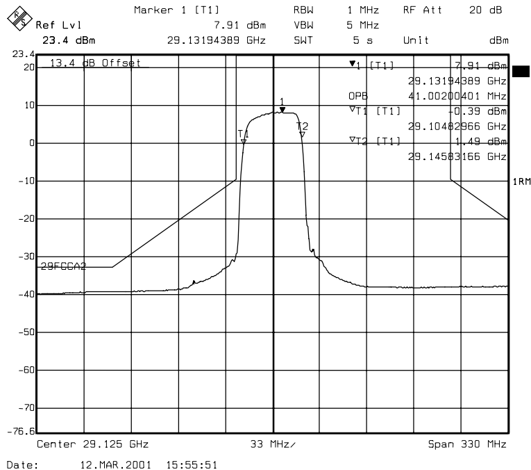
Figure 2. 32 QAM, taken in block A2 (low end), Actual Output Power 23.46 dBm
