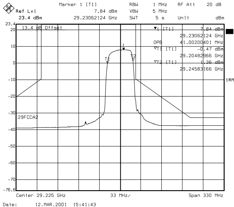
Figure 6. 32 QAM, taken in block A2 (high end), Actual Output Power 23.23 dBm
