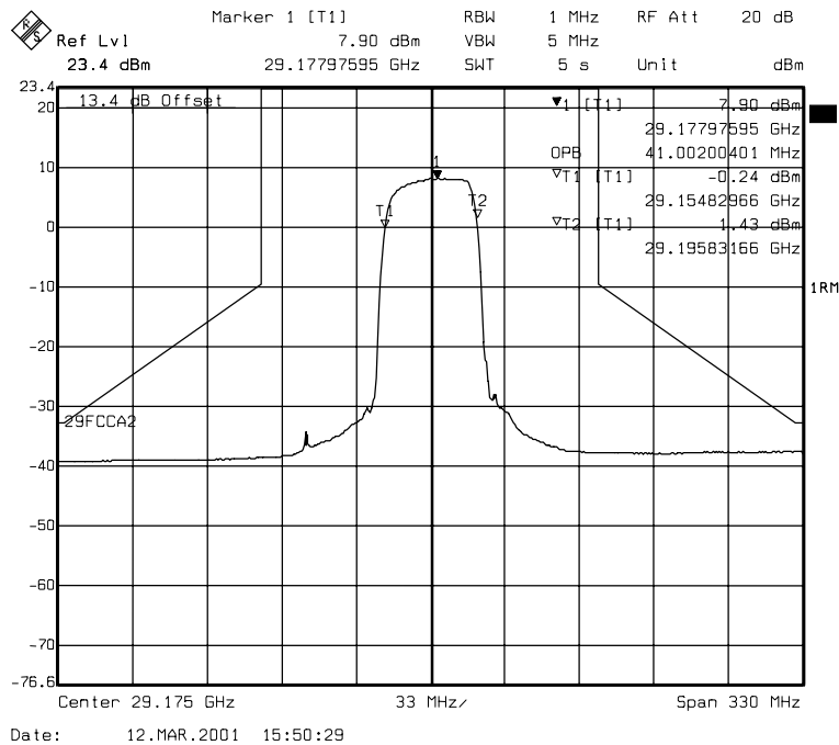
Figure 4. 32 QAM, taken in block A2 (mid), Actual Output Power 23.25 dBm
