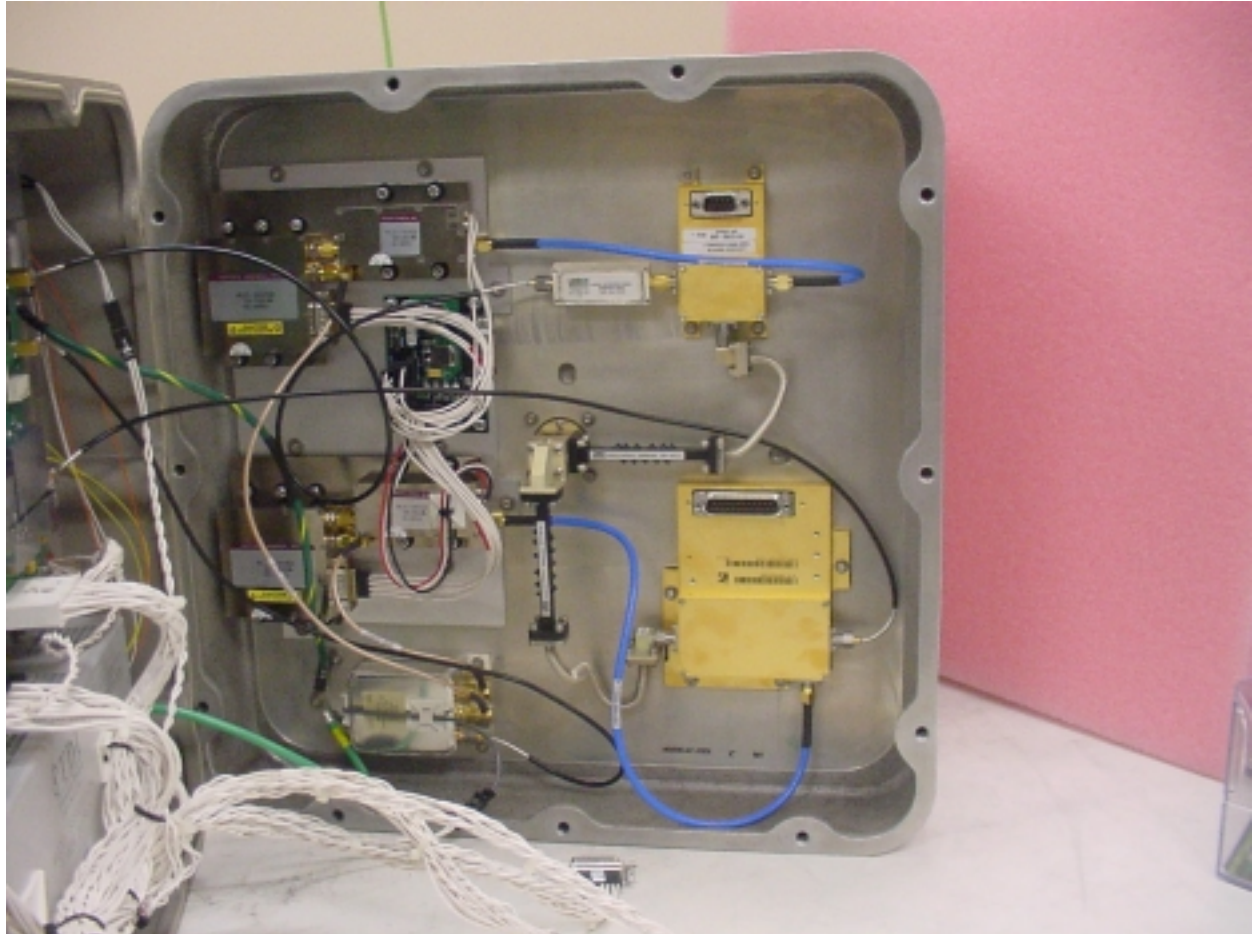
Internal photograph of transmitter, receiver, synthesizer, and filter/attenuator section
