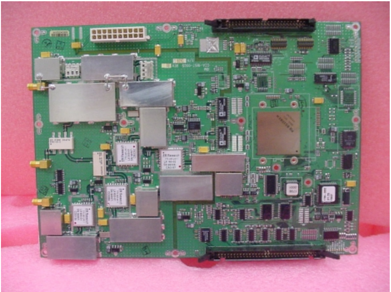
Top view Modem board
