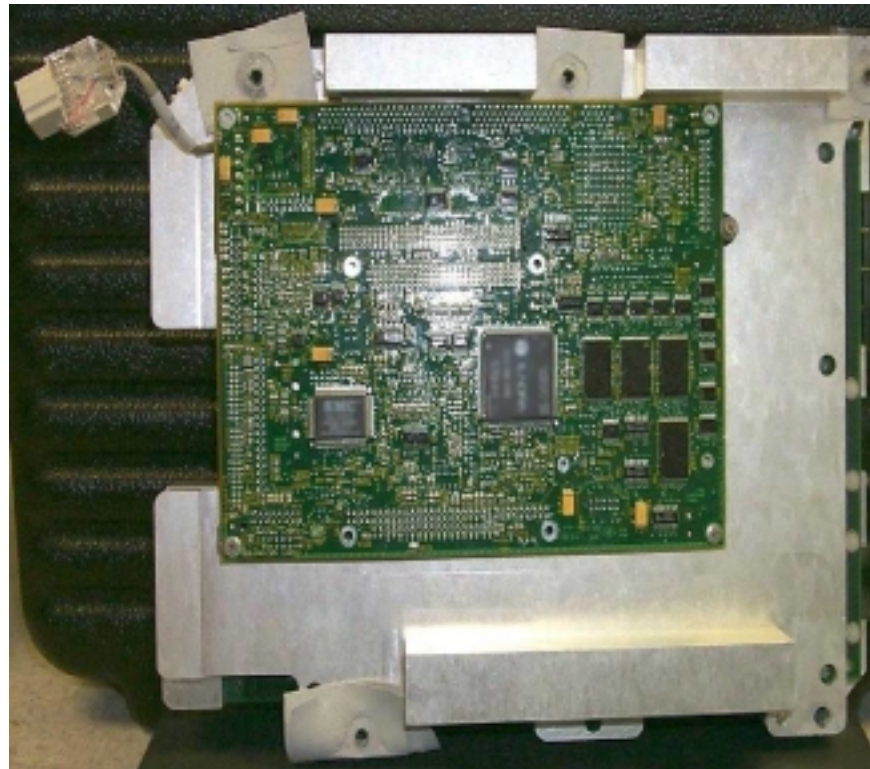
Bottom view of CPU board with heat sink attached, top view of CPU board
