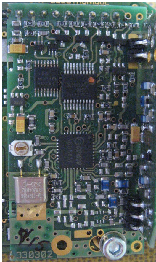
Emitter, radio module, front side
