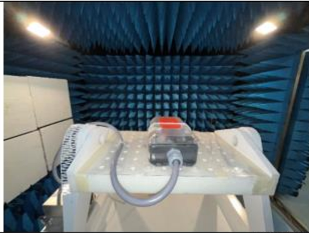
Test setup under 1GHz
