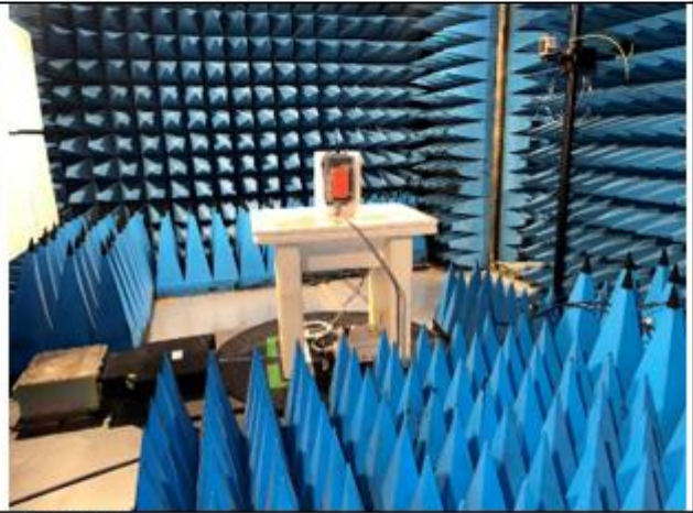
Test setup under 1GHz
