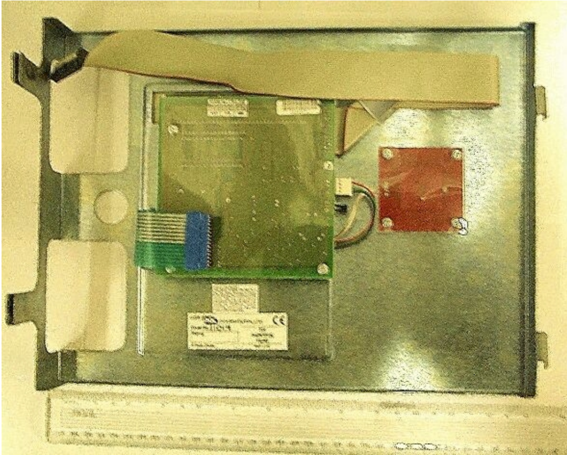
Rear View of Both PAC and READYKEY Variants (NOTE: The colour of the square PCB to the right hand side is due to red solder resist. This colour will change to green for future production)
