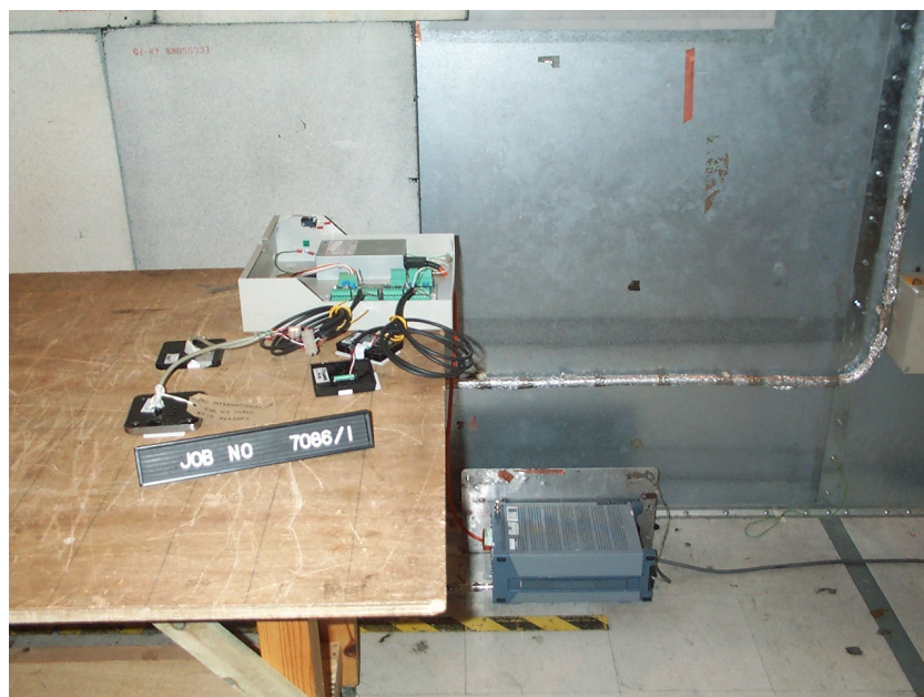
Conducted RF Emission (14/15/02/2006)
