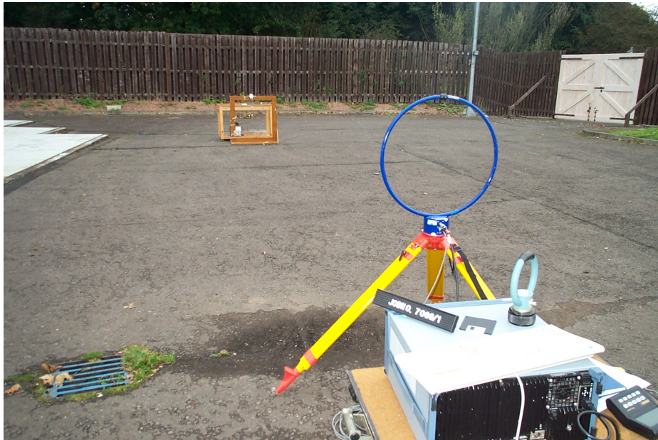
Radiated Emission <30MHz
