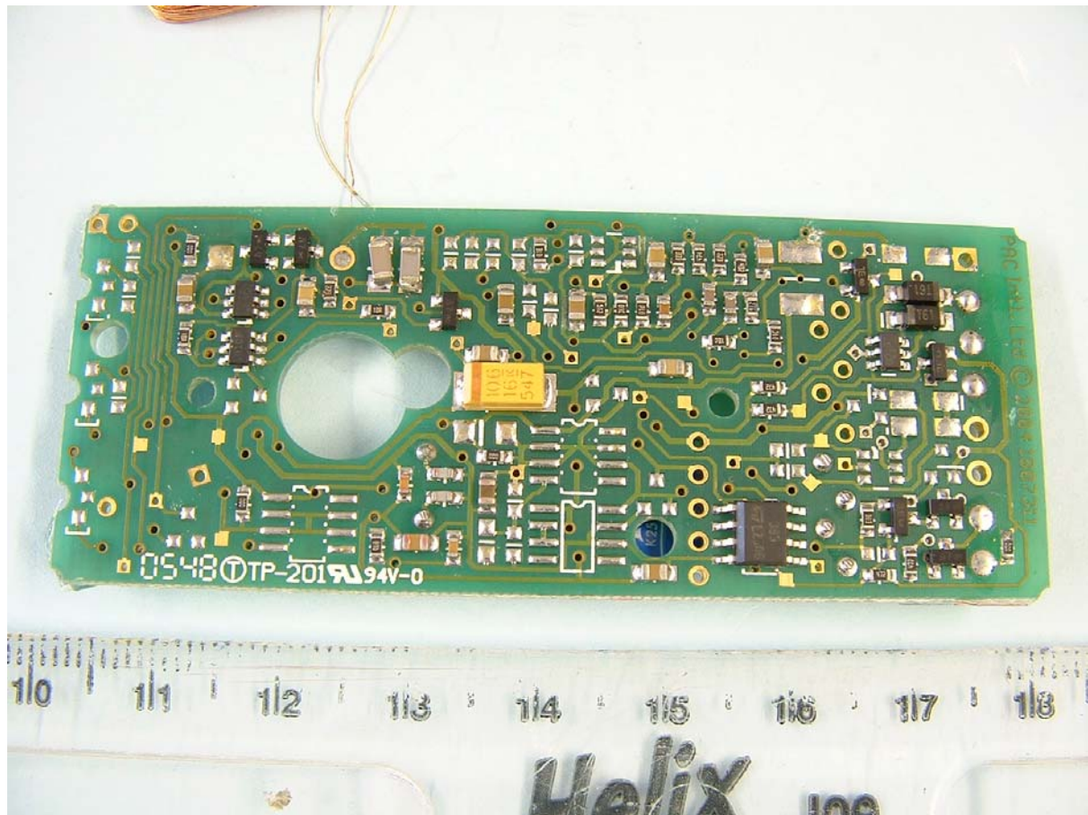
Internal Photo 5 of 7 – RFID reader PCB, side 2 view.
