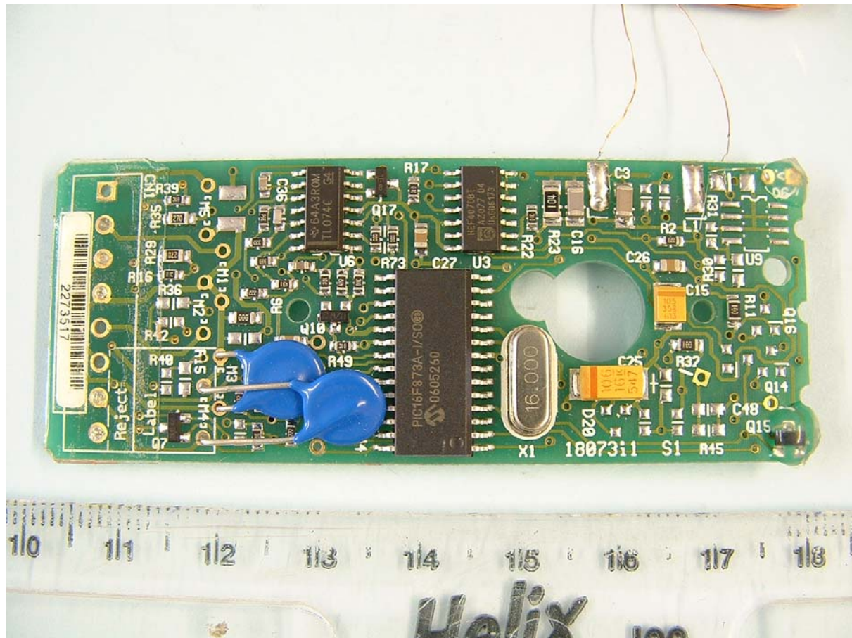
Internal Photo 4 of 7 – RFID reader PCB, side 1 view.
