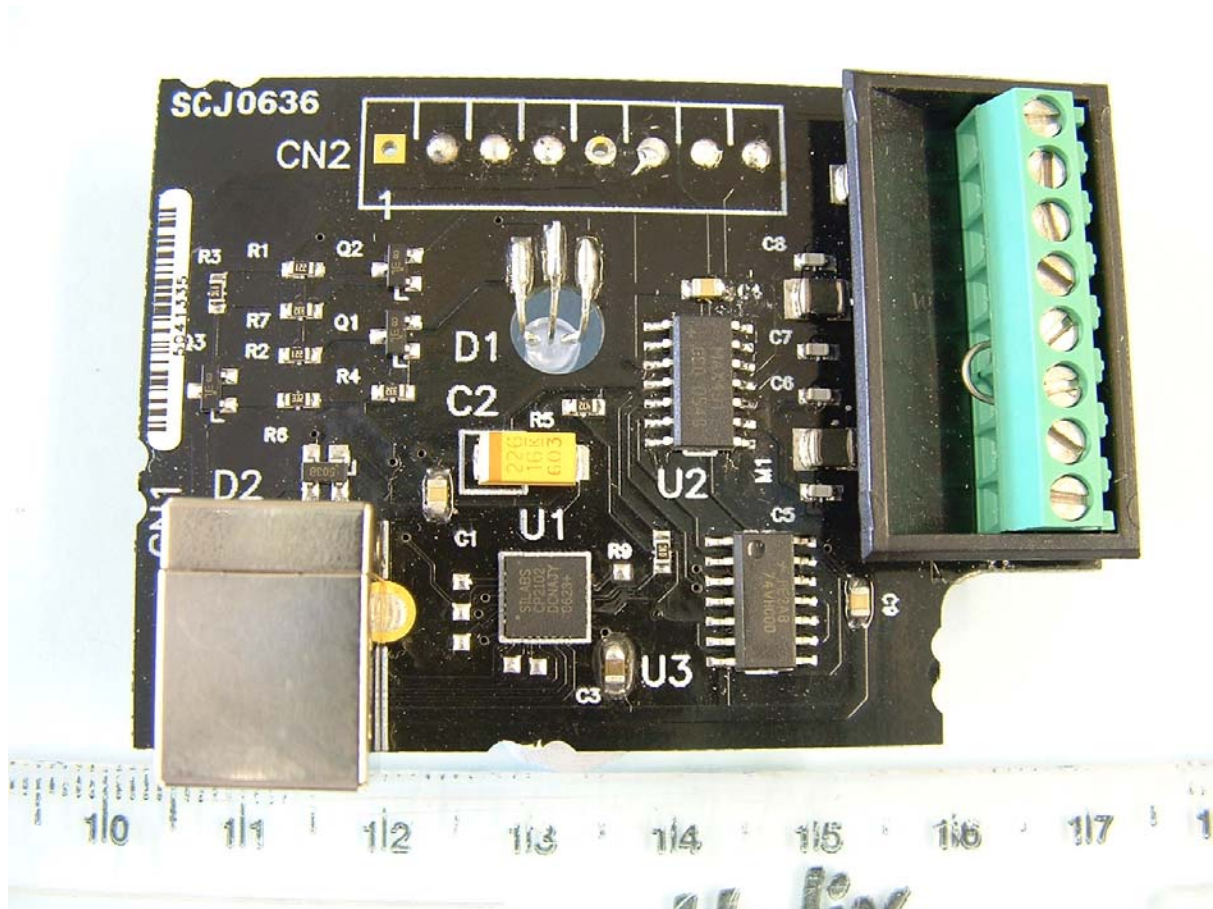
Internal Photo 2 of 7 – USB interface PCB, component side view.
