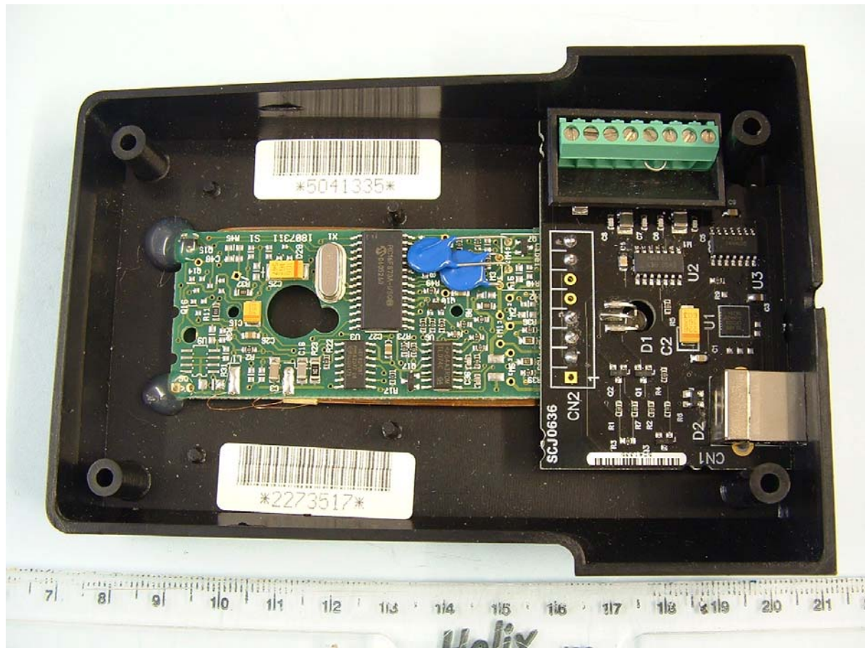
Internal Photo 6 of 7 – Internal assembly view unpotted.
