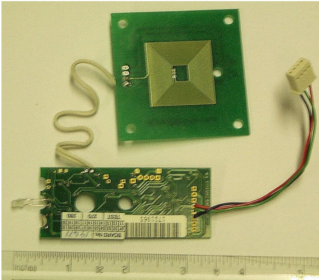
Reader PCB Assembly (Solder side)
