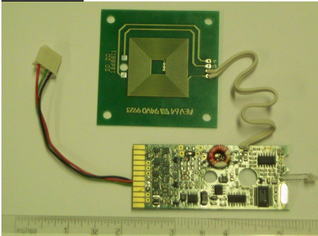
Reader PCB Assembly (Component Side)
