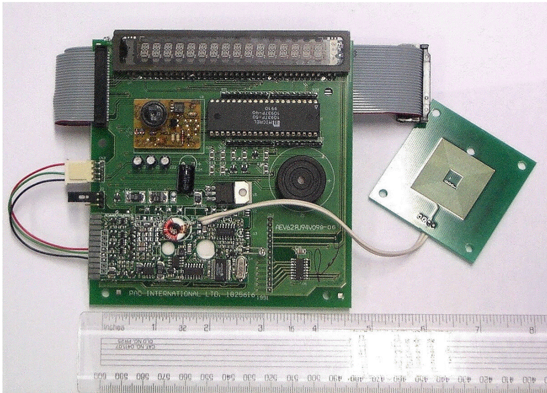
Main board PCB Assembly (Component Side)
