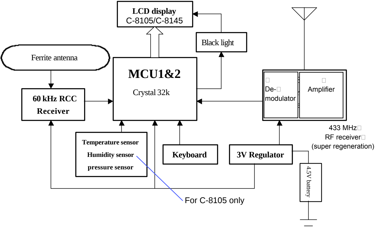
Figure 1 C-8105 Block diagram C-8145
