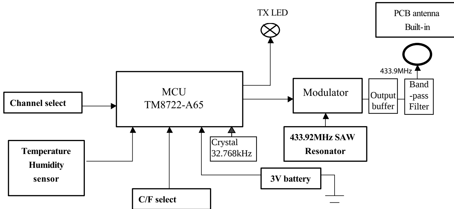
Figure 1 C8201(FCC) Block diagram
