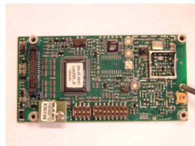
RADIO BOARD
