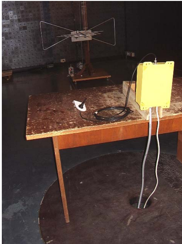
Radiated Emission:
