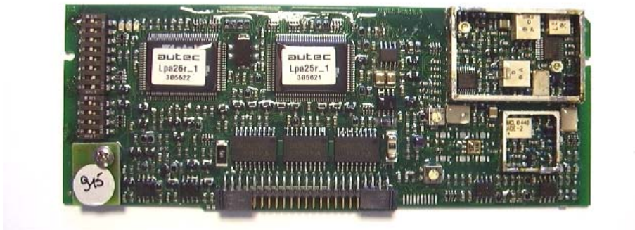
Radio Module without shield
