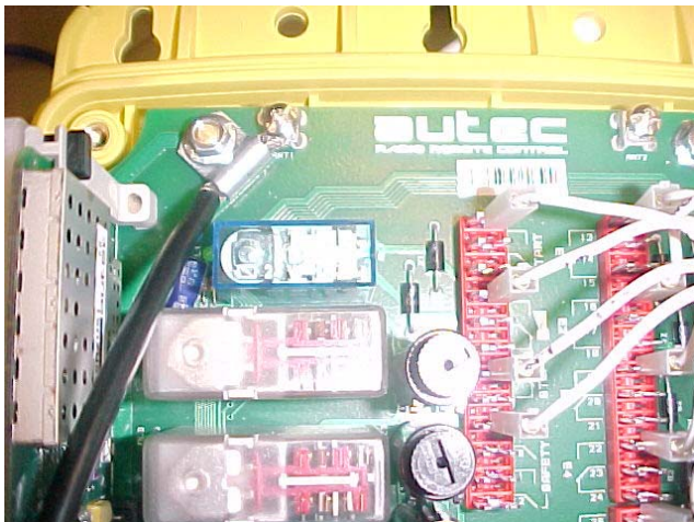
DEDICATED ANTENNA
