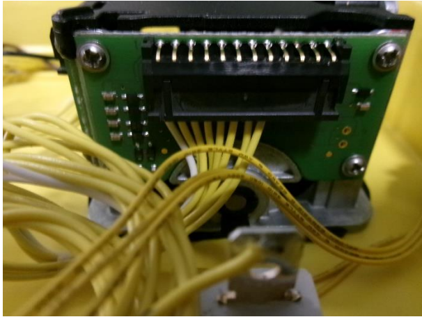
Joystick PCB
