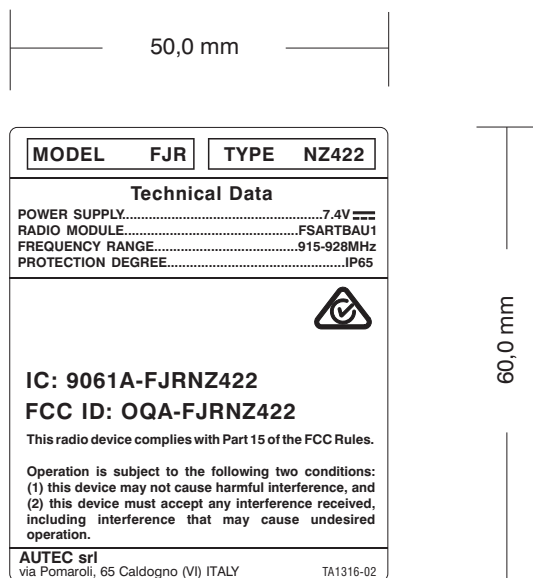
FJR label and its dimension
