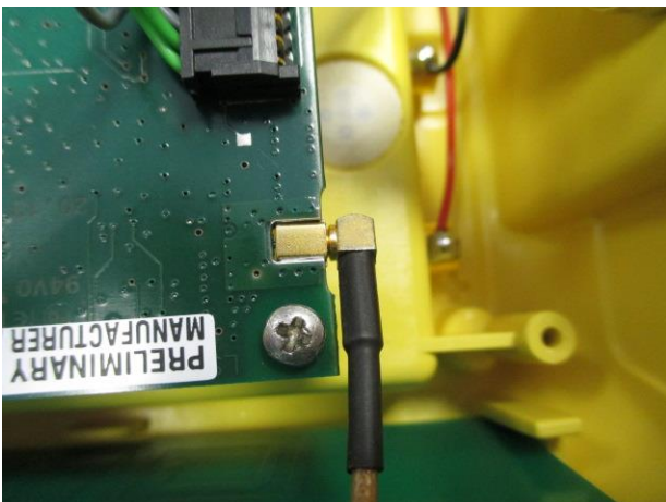
Antenna connectors:
