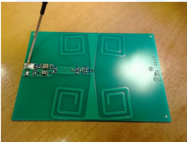
Antenna connectors:
