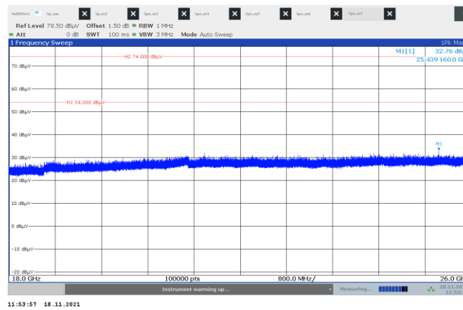
Figure 8.6-10: Radiated spurious emissions 18–26 GHz
