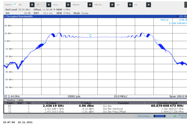
Figure 8.4-2: 99% occupied bandwidth
