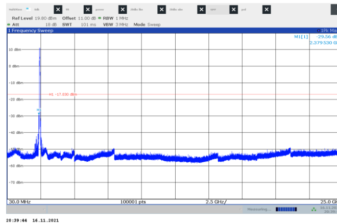
Figure 8.6-3: Conducted spurious emissions
