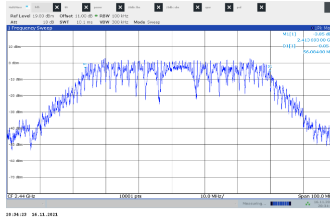
Figure 8.4-1: 6 dB bandwidth
