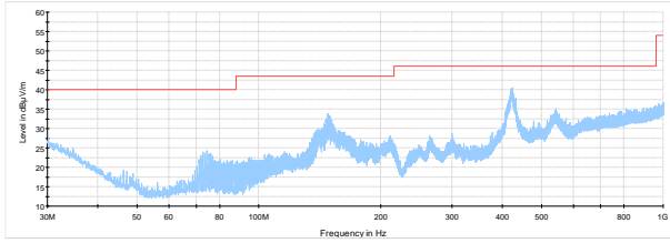
Figure 8.6-8: Radiated spurious emissions 30–1000 MHz
