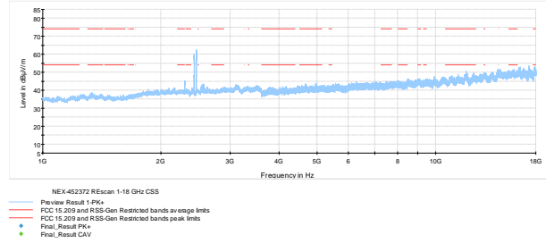
Figure 8.6-9: Radiated spurious emissions 1–18 GHz
