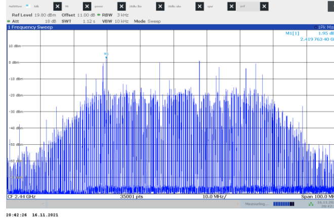
Figure 8.7-1: PSD
