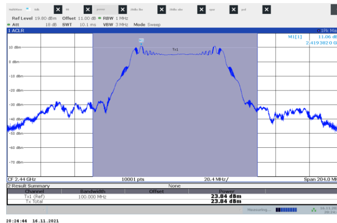
Figure 8.5-1: Output power
